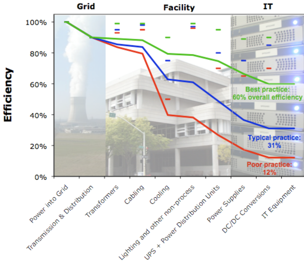
Figure 3. Individual (dashes) and cumulative (curves) efficiencies of data center systems. The system boundary shown here does not include "upstream" efficiencies in power generation, which are about 35%, or downstream losses and parasitic energy (e.g. fans) within the IT equipment itself.
