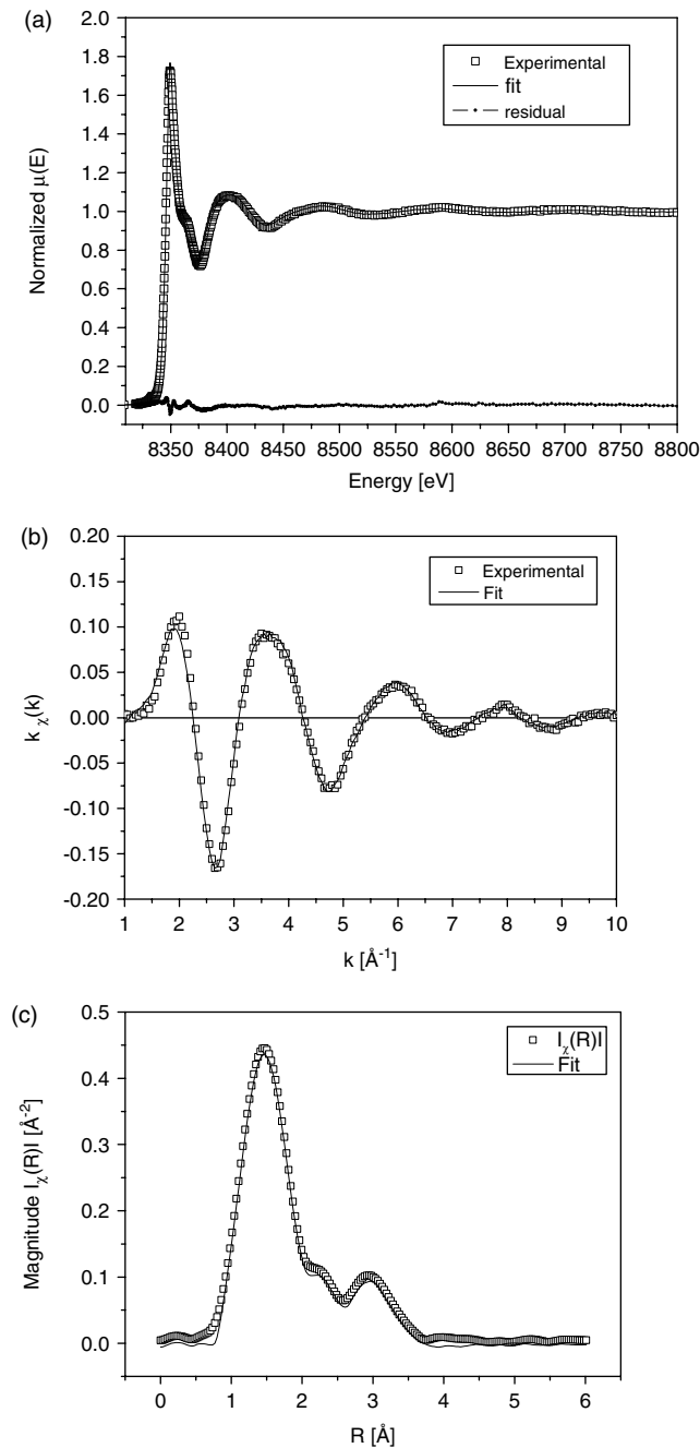
Figure 4. The fit result for normalised x-ray absorption spectra at Ni-K absorption edge from the leaf of S. tryonii for 61% citrate; 30% phosphate and 9% histidine; plotted against (1) energy; (2) wave vector k and (3) relative distance R of scatterer from the Ni absorber.
