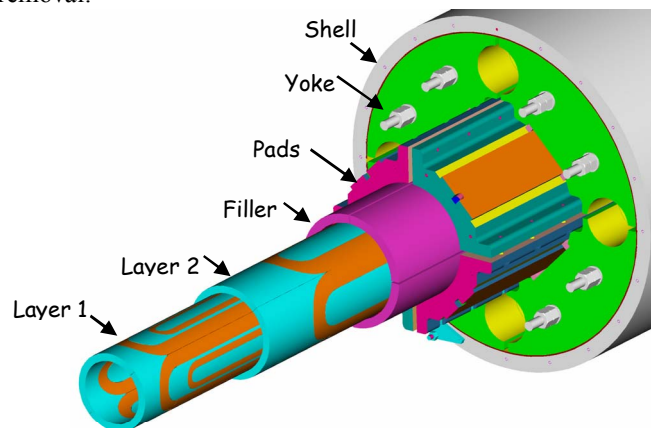
Fig. 2. View of coils and supporting structure
