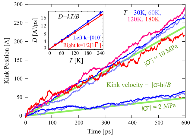
Fig. A.23. Results of kink drift simulations for \mathbf{k} = 1/2[1\bar{1}1] (right) kinks on 1/2\langle 111 \rangle\{10\bar{1}\} screw dislocations. We see a temperature independent drift velocity v_k = |\boldsymbol{\sigma} \cdot \mathbf{b}|/B in very good agreement with B determined from zero stress kink diffusion simulations (green lines). Inset: Results from kink diffusion simulations. We see the diffusivity D = kT/B rises linearly with temperature, meaning that B is independent of temperature.
