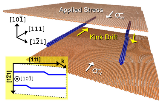
Fig. A.22. Illustration of kink drift simulations. Kinks on a 1/2\langle 111 \rangle\{10\bar{1}\} screw dislocation dipole, characterized by a lattice ‘kink’ vector \mathbf{k} , are subject to an applied stress on bounding (10\bar{1}) planes. Under no applied stress with fully periodic boundary conditions the kinks diffuse freely. Inset: Cartoon of the supercell along [10\bar{1}] , illustrating the relation of the kink vector to a kinked dislocation line.
