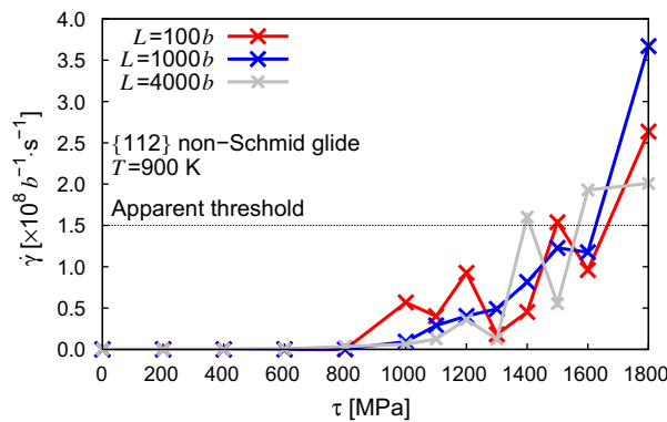
Fig. 17. Debris loop generation rate at 900 K during {112} non-Schmid conditions for three different initial dislocation lengths. The apparent threshold above which self-pinning is seen to dominate the kinetics is marked with a dashed line.
