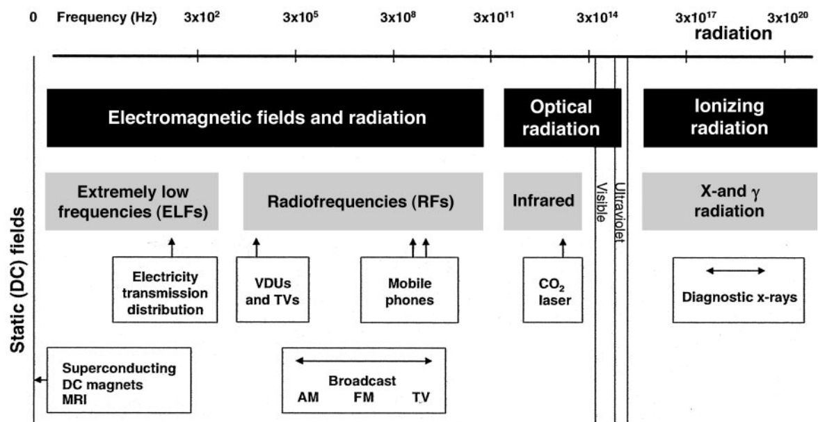
Fig 1. Electromagnetic spectrum. VDUs indicates video display units.
