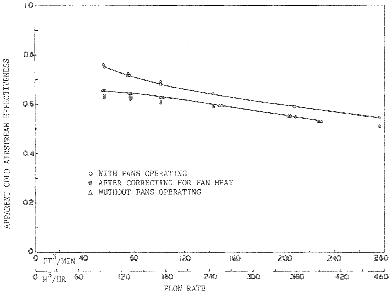
FIGURE 20. APPARENT COLD AIRSTREAM EFFECTIVENESS VERSUS FLOW RATE FOR THE FLAKT RDA heat EXCHANGER
