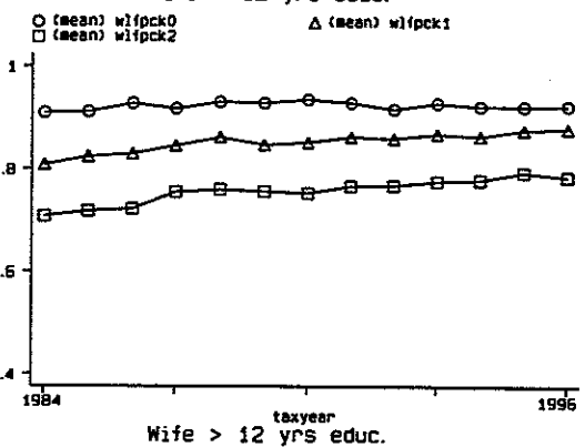
Wife's labor force participation
