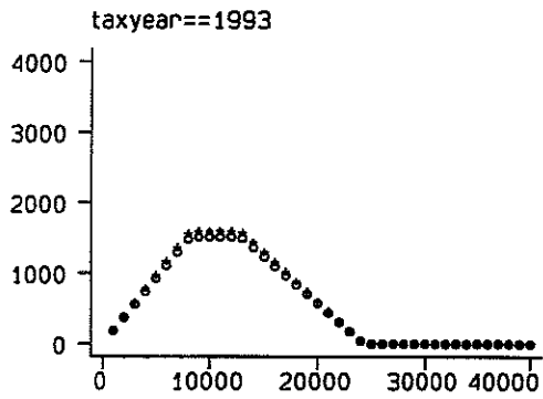
1995$ EITC benefit, by family earnings
