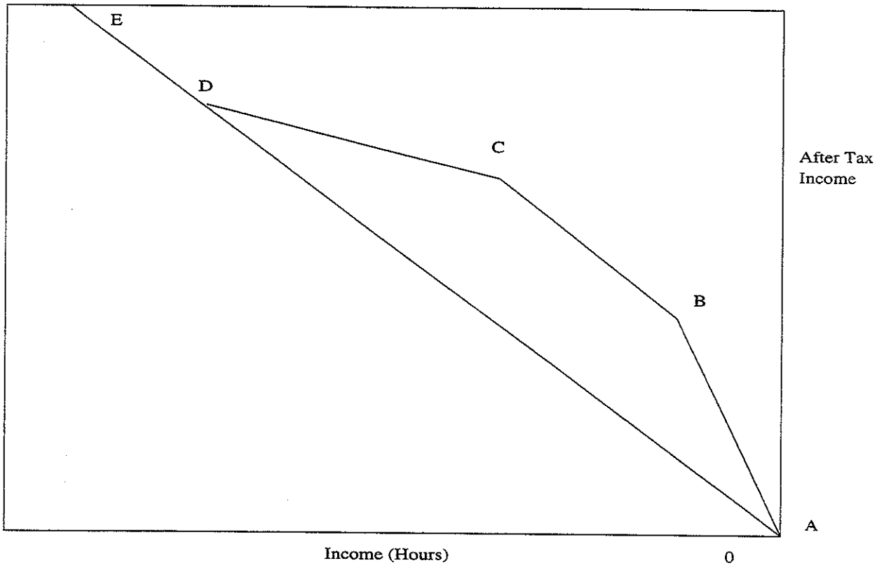
Figure 1: EITC Budget Constraint
