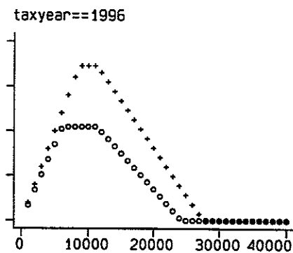
1995$ EITC benefit, by family earnings
