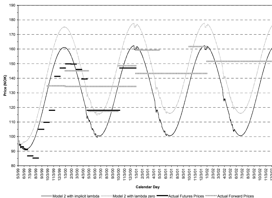
B) Model 2 Theoretical Prices vs. Actual Market Prices (5/03/1999)
