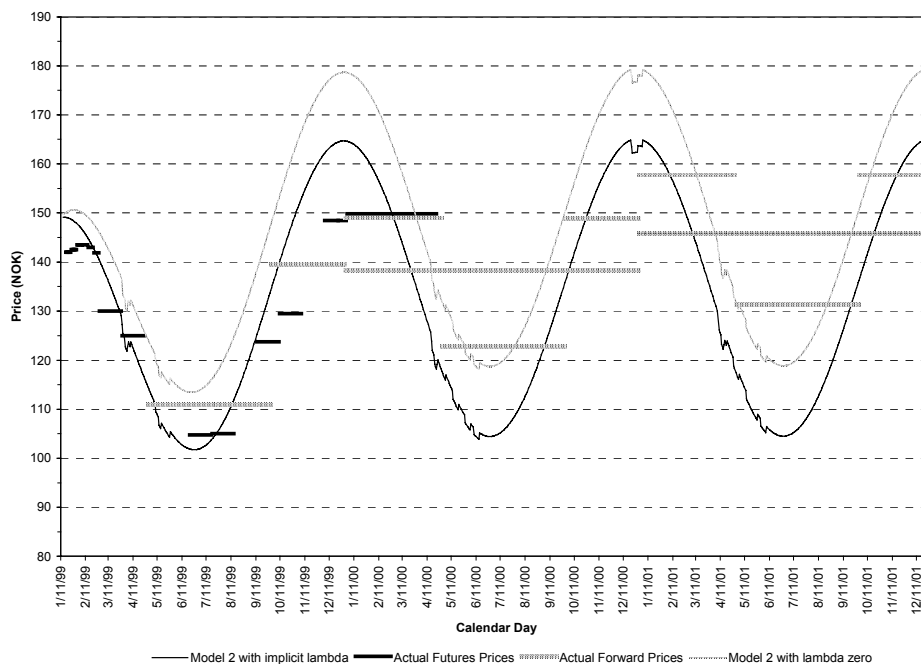
B) Model 2 Theoretical Prices vs. Actual Market Prices (5/03/1999)
