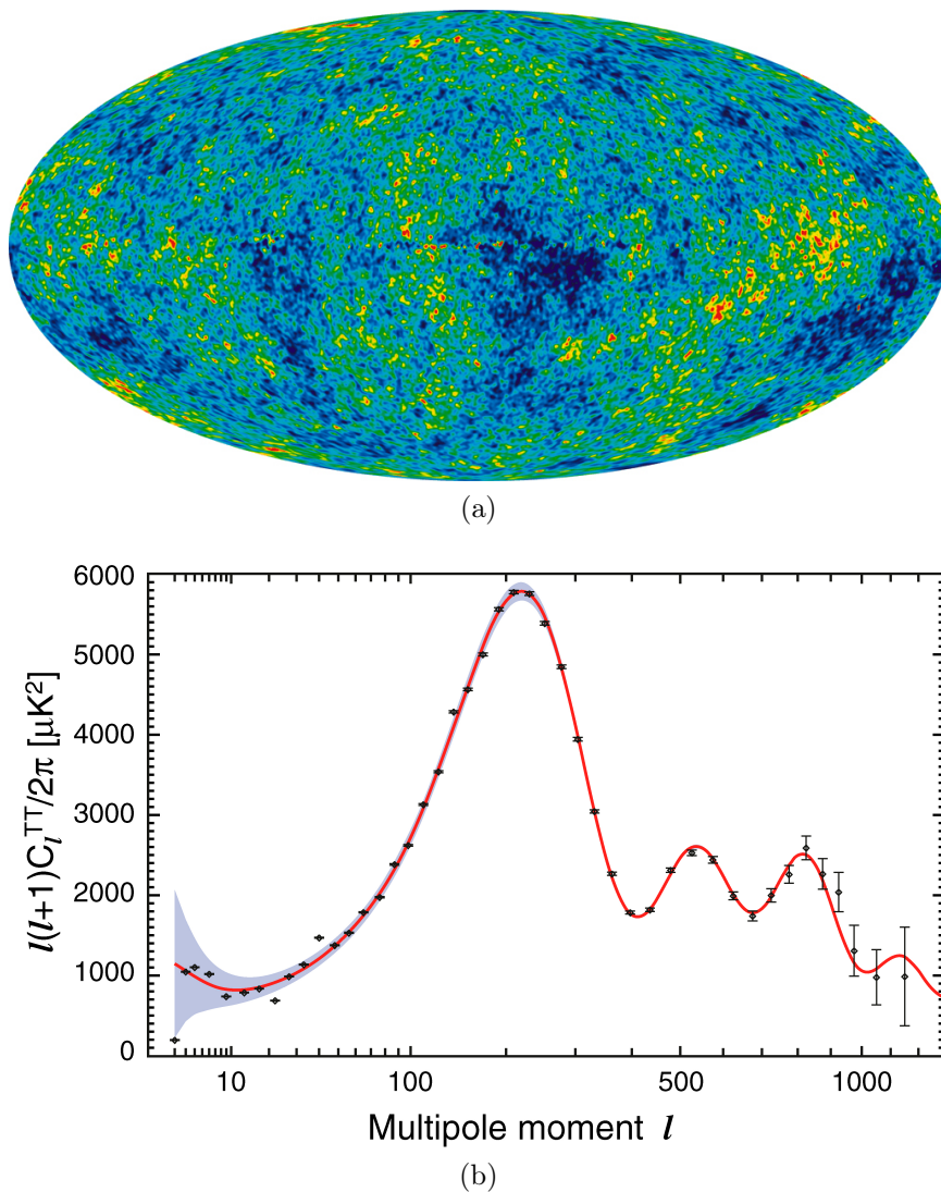
Figure 1.7: WMAP 7-year data. (a) WMAP observed temperature map across the full sky. Here, the color scale is set in reference to the 2.7 Kelvin average temperature. The range of the color scale is \pm 200 \mu\text{K} . This map is a linear combination of maps taken at five wavelengths to minimize galactic foreground emission. ( Internal Linear Combination Map, courtesy of WMAP Science Team ) (b) The temperature map was decomposed into spherical harmonics, and fluctuation power is plotted as a function of multipole moment (the reciprocal of spot size). [56].
