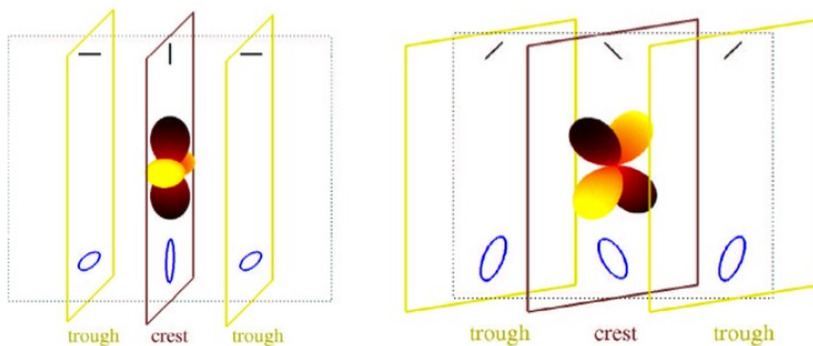
(b) Tensor perturbation
