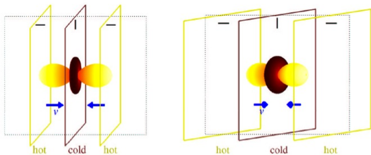
(a) Scalar perturbation
