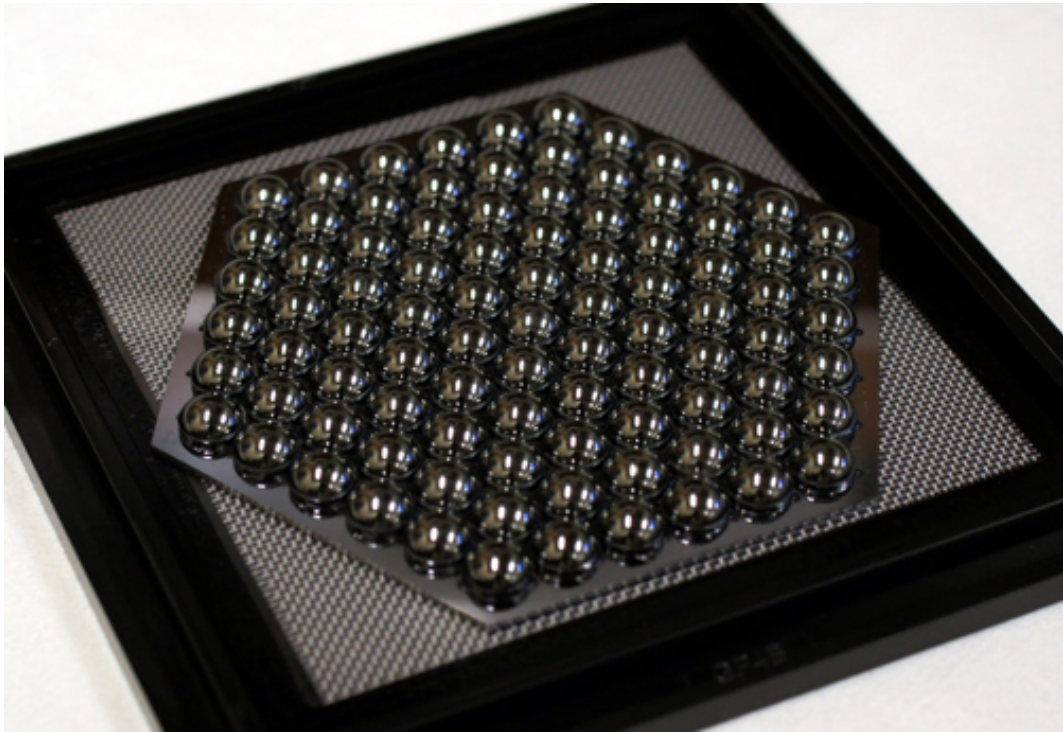
Figure 4.13: Completed Array.
