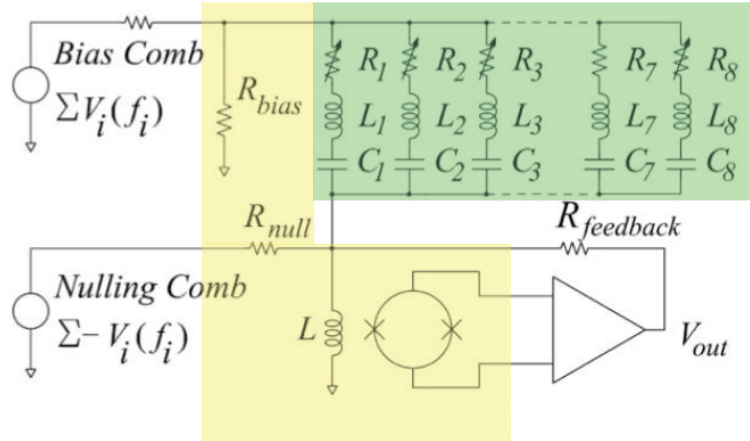
Figure 3.11: Frequency Multiplexing Schematic. The green shaded region shows the bolometers each in series with an LC filter. Eight of the filter/detector pairs are wired in parallel and receive a comb of bias frequencies, shown on the upper left. The components shown here in green all reside on a single LC circuit board, except for the bolometers labeled R1 through R8 which reside on the detector wafer. The eight bolometers are read out with a single SQUID amplifier, shaded yellow in this figure (where eight SQUIDS reside on a single SQUID board).
