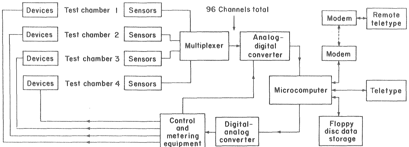
Fig. 3. Mobile Window Thermal Test Facility Instrumentation.
