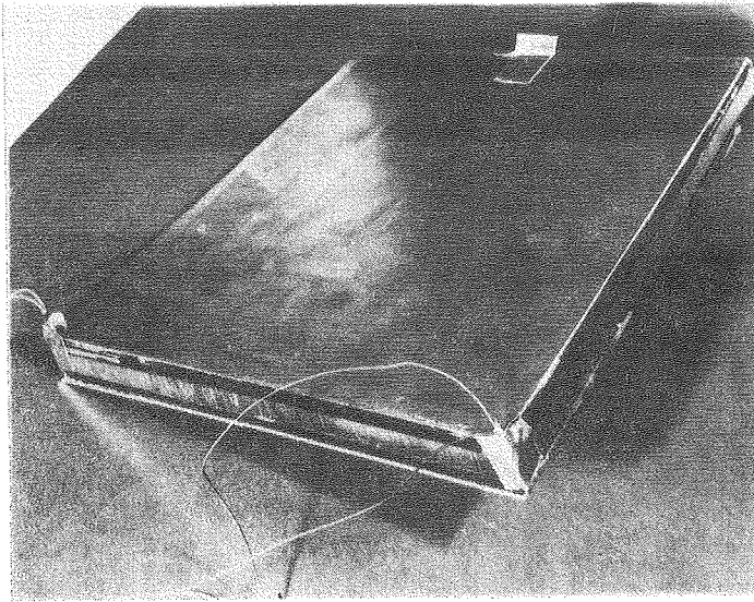
Fig. 5. Prototype Heat Flow Meter. Overall size is 30cm X 30cm (1 ft X 1 ft).
