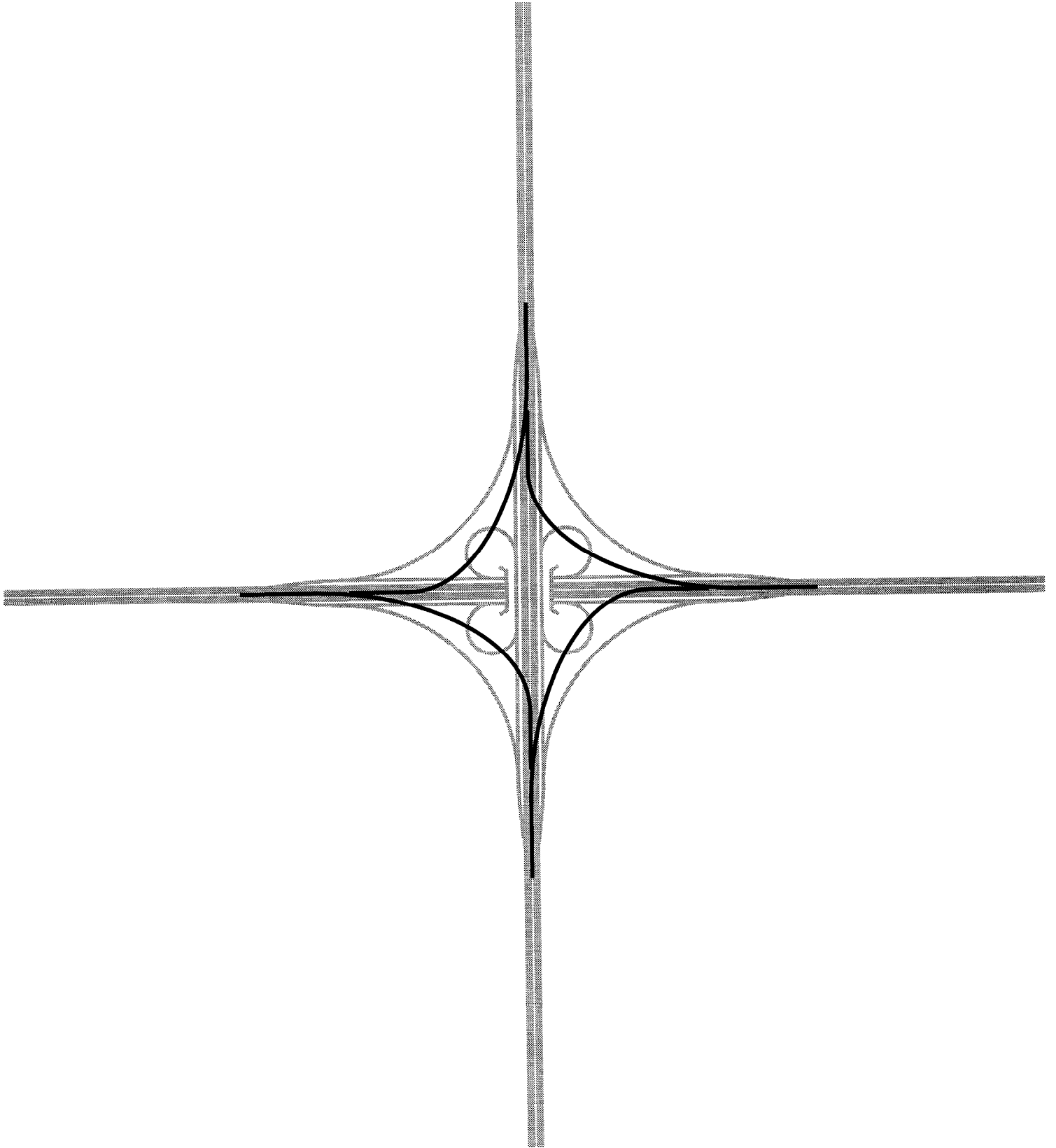
Figure 1. A Bird's-Eye View of the Staggered-Diamond Design.
