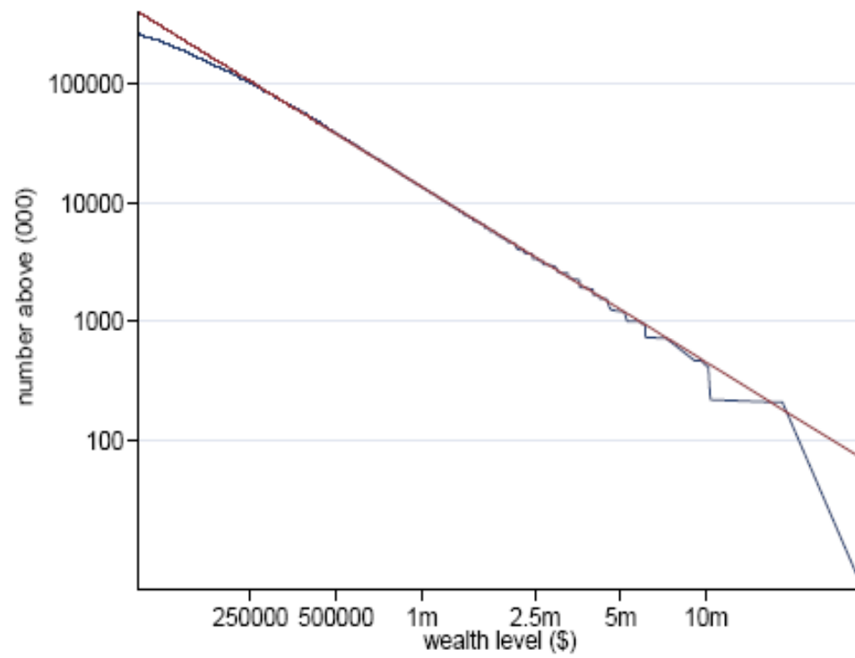
Fitted Pareto Distribution
