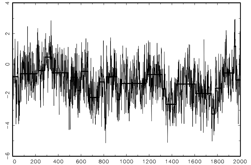
Figure 4-4. I(d) process ( d=0.8 ) and Estimated Level Shifts
