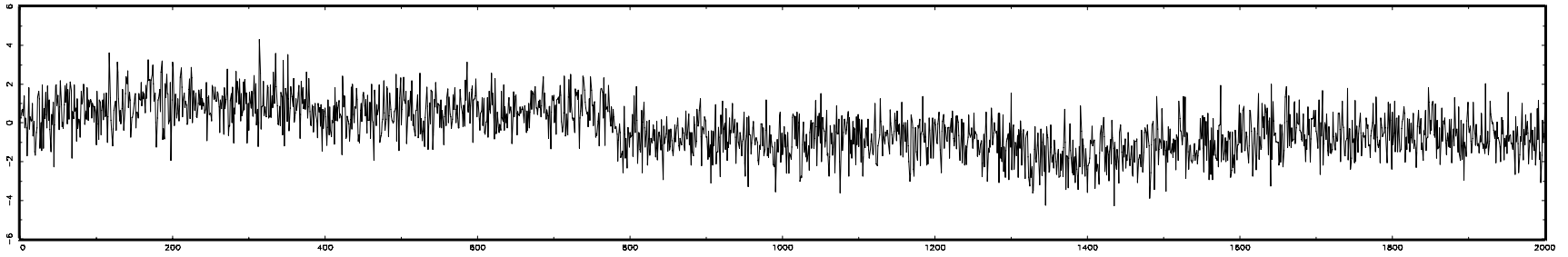
Figure 2-2: Break Points (Binomial Distribution)
