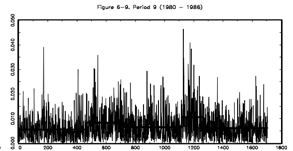
Figure 6. Absolute Stock Return and Breaks of 10 Sub-Periods in 1/4/1928-8/30/1991
