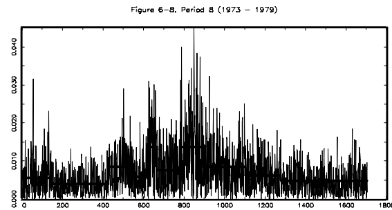
Figure 6. Absolute Stock Return and Breaks of 10 Sub-Periods in 1/4/1928-8/30/1991
