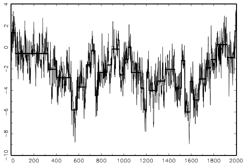
Figure 4-3. I(d) process ( d=0.6 ) and Estimated Level Shifts
