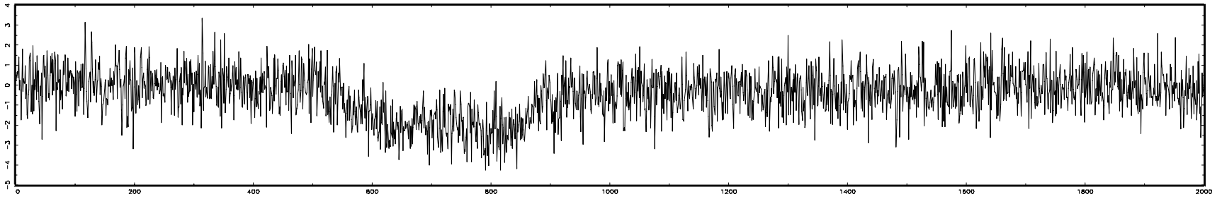
Figure 3-2: Break Periods (Markov Switching Process)
