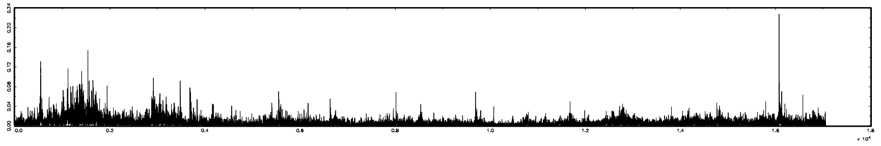
Figure 5-3: S&P 500 Daily Absolute Returns (Moving Averaged with 220 days)
