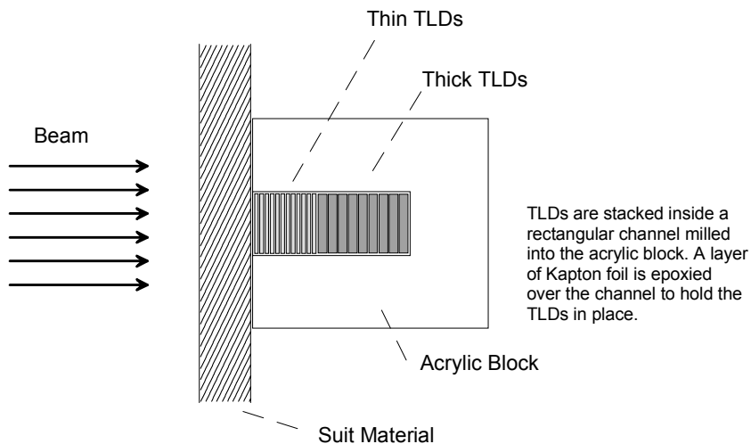
Figure 2. TLD Stack used in making dose/depth measurements behind EVA suit material and helmets exposed to 6 MeV electrons and 60 MeV protons.
