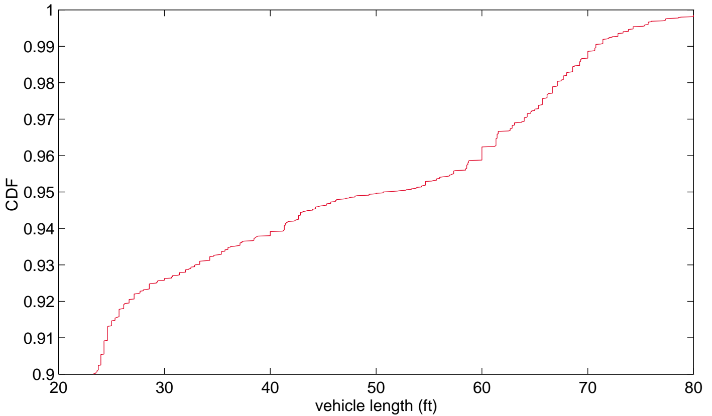
FIGURE 4-13 B: Detail of the CDF from part A, showing the large range of lengths observed in the longest 10 percent of the vehicles.
