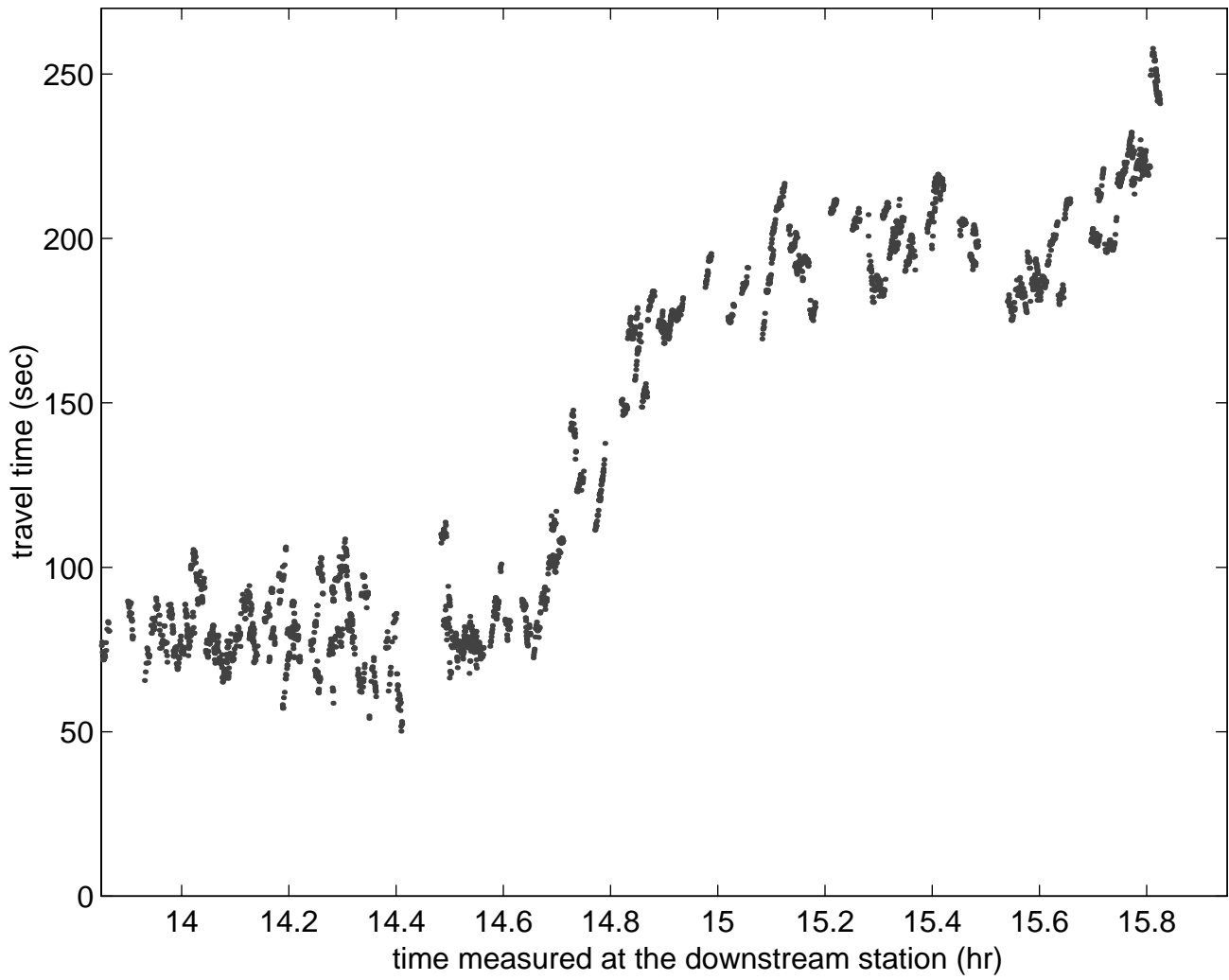
FIGURE 5-8: Travel times for matched vehicles using the Approximation Algorithm.
