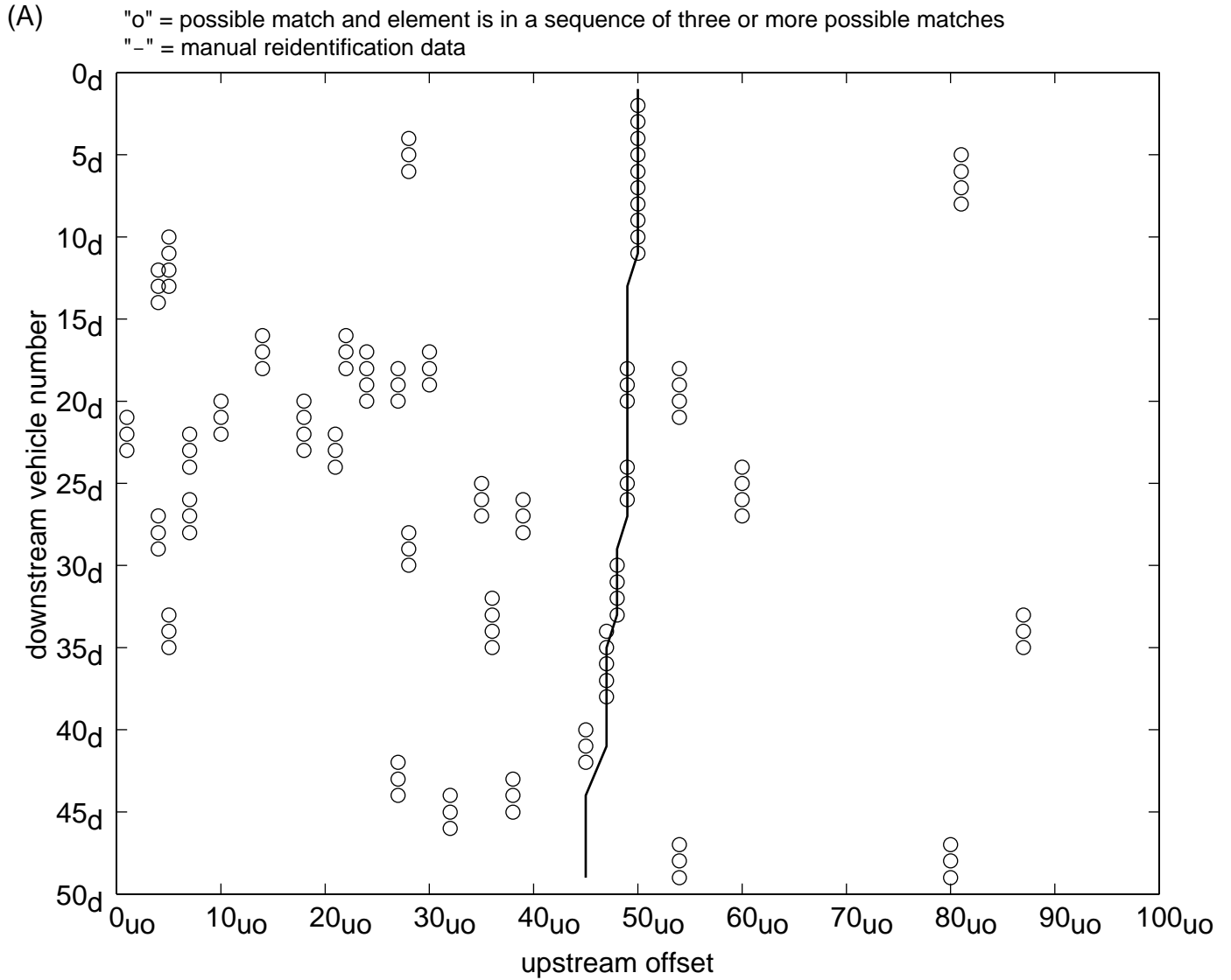
FIGURE 4-19: (A) Filtered offset match matrix, retaining all platoons of three or more vehicles, (B) Localizing the offset between the upstream and downstream by calculating the column average weights from filtered offset match matrix
