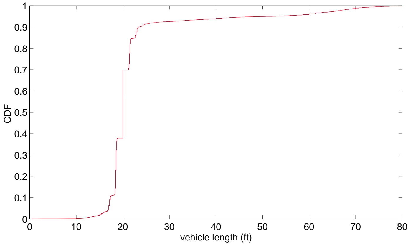
FIGURE 4-13 A: Cumulative Distribution of measured vehicle lengths in one lane during the evening peak at a detector station. Sample size = 8002 vehicles
