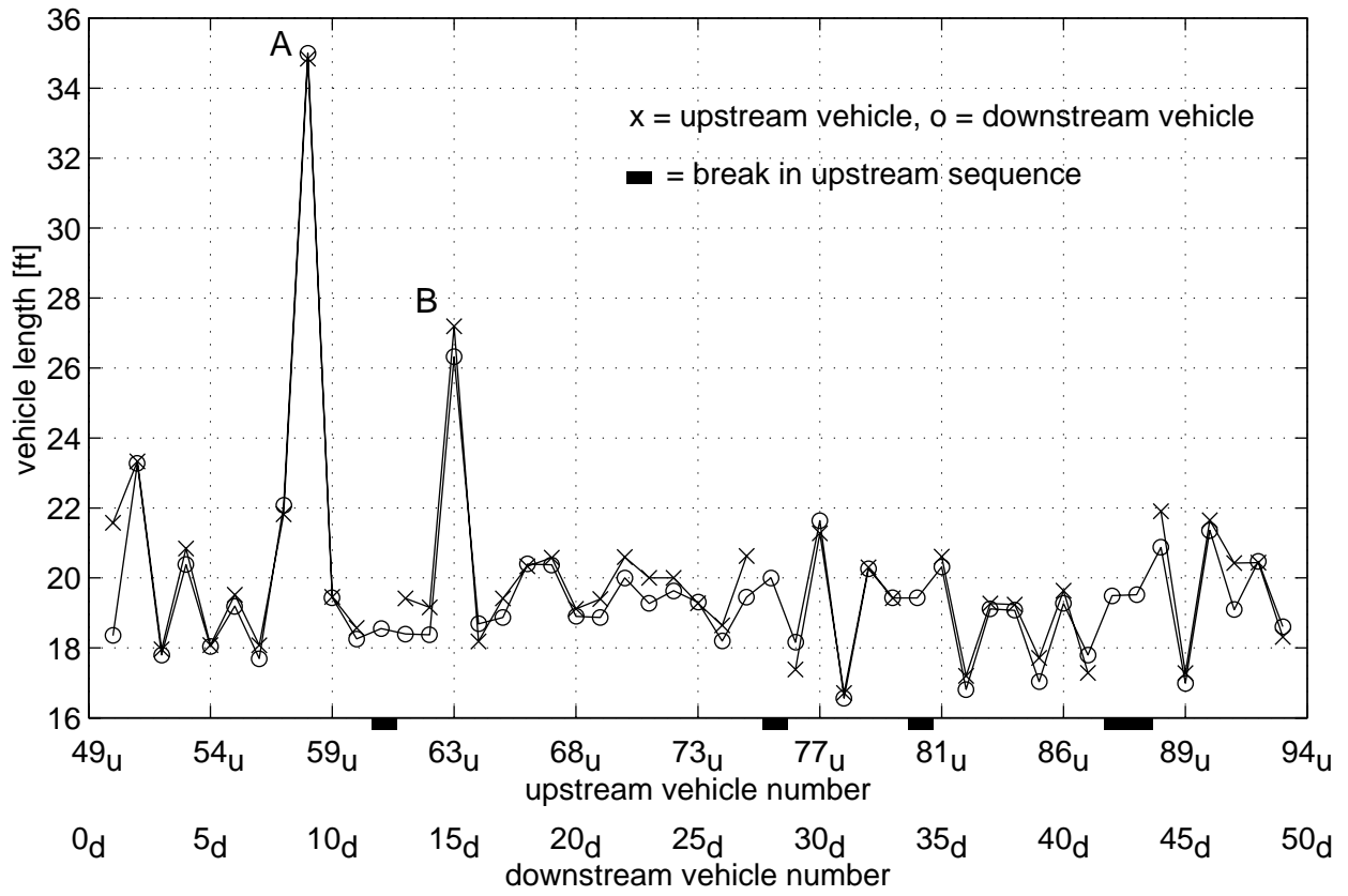
FIGURE 4-4A: Manual reidentification, superposition of the vehicle lengths from Figure 4-2
