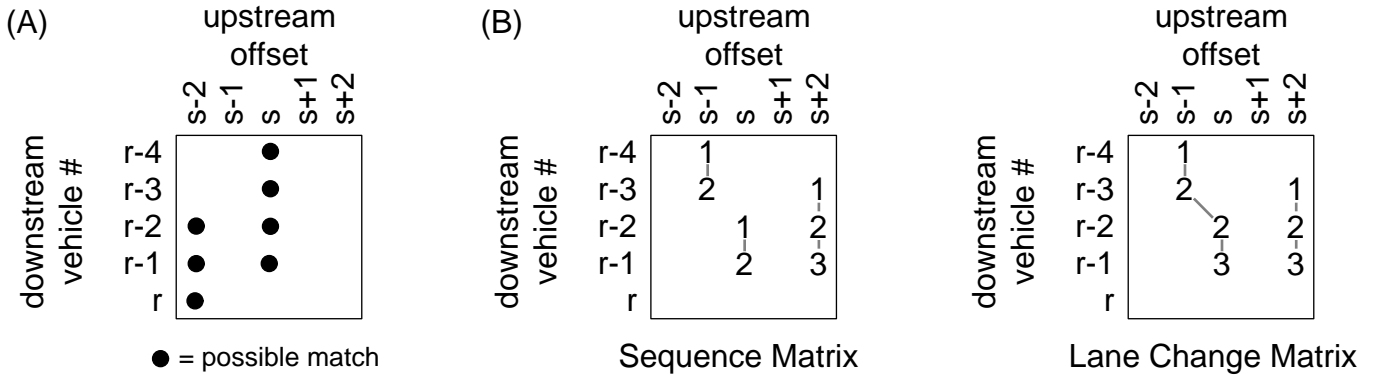
FIGURE 9-2: (A) The end of the sequence in column s can only be detected after the first unlikely element has been observed in the column. In this case once vehicle r passes the downstream station. (B) This figure shows a simple example of how to differentiate between sequences in the lane change matrix that do not contain a lane change from those that do. If the sequence does not contain a lane change, the ending value will be identical to the sequence matrix (e.g., element (r-1, s+2) ), otherwise, it will be greater (e.g., element (r-1, s) ).
