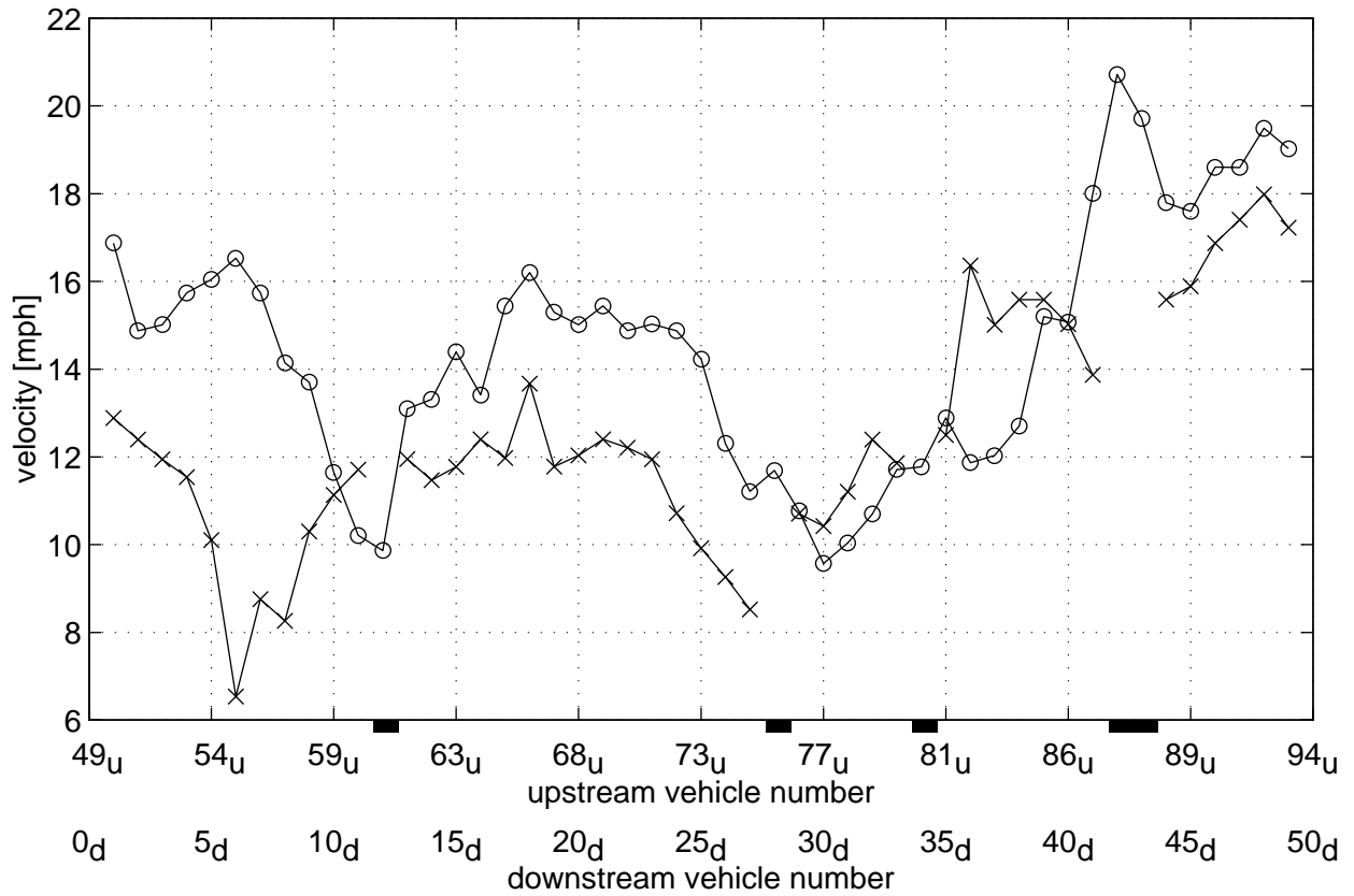
FIGURE 4-4B: The corresponding measured vehicle velocities
