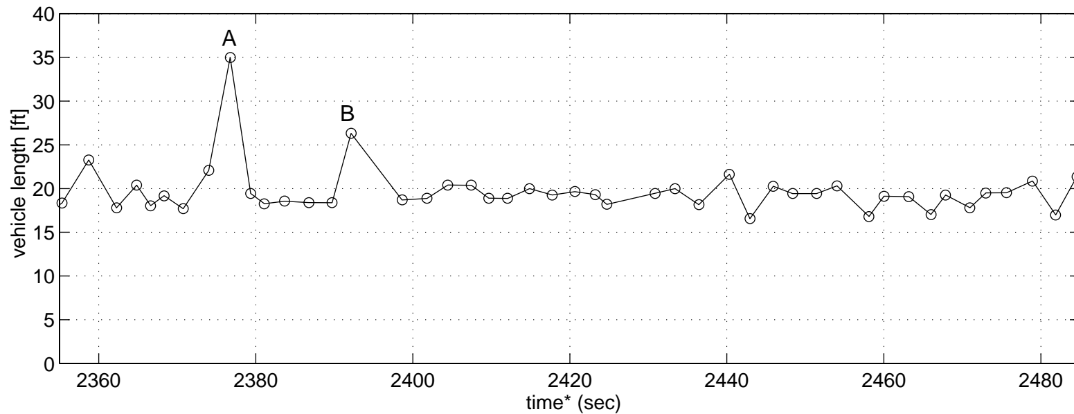
FIGURE 4-2B: Detail of the downstream vehicle length time series
