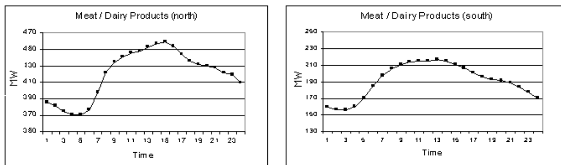
Figure 6.8. Load profiles during a peak day for a meat/dairy industry; Northern and Southern California
