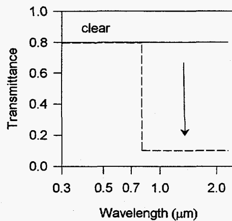
Fig. 1. Idealized electrochromic spectra in the "clear" and "darkened" state: (a) uniform switching occurs over the entire solar spectrum; (b) switching occurs over the visible spectrum only with constant low transmission in the near infrared in both "clear" and "dark" states; and (c) switching occurs over the infrared spectrum only with constant high transmission in the visible spectrum in both "clear" and "dark" states.
