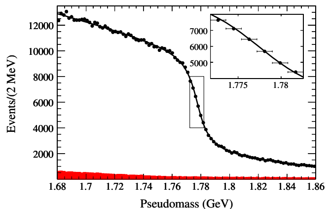
FIG. 8 (color online). Combined \tau^+ and \tau^- pseudomass endpoint distribution. The points show the data, the curve is the fit to the data, and the solid area is the background. The inset is an enlargement of the boxed region around the edge position showing the fit quality where p_1 is most sensitive.
