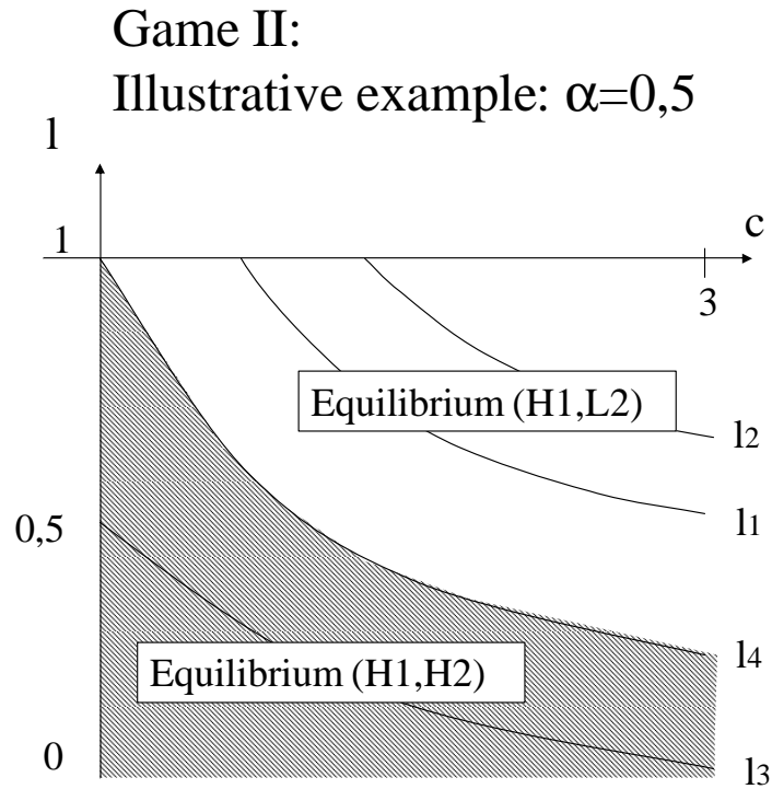
Figure 2: Thresholds in Game (II) for \alpha = \frac{1}{2}
