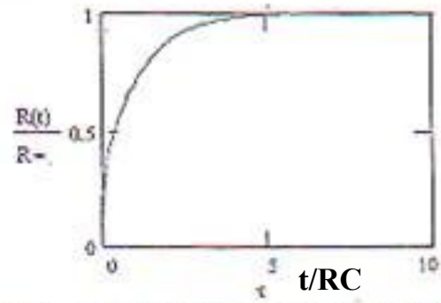
Figure 3. The time required to achieve steady state resistance during constant current cycling. At one time constant, \tau , the resistance is at 70% of its steady state value.
