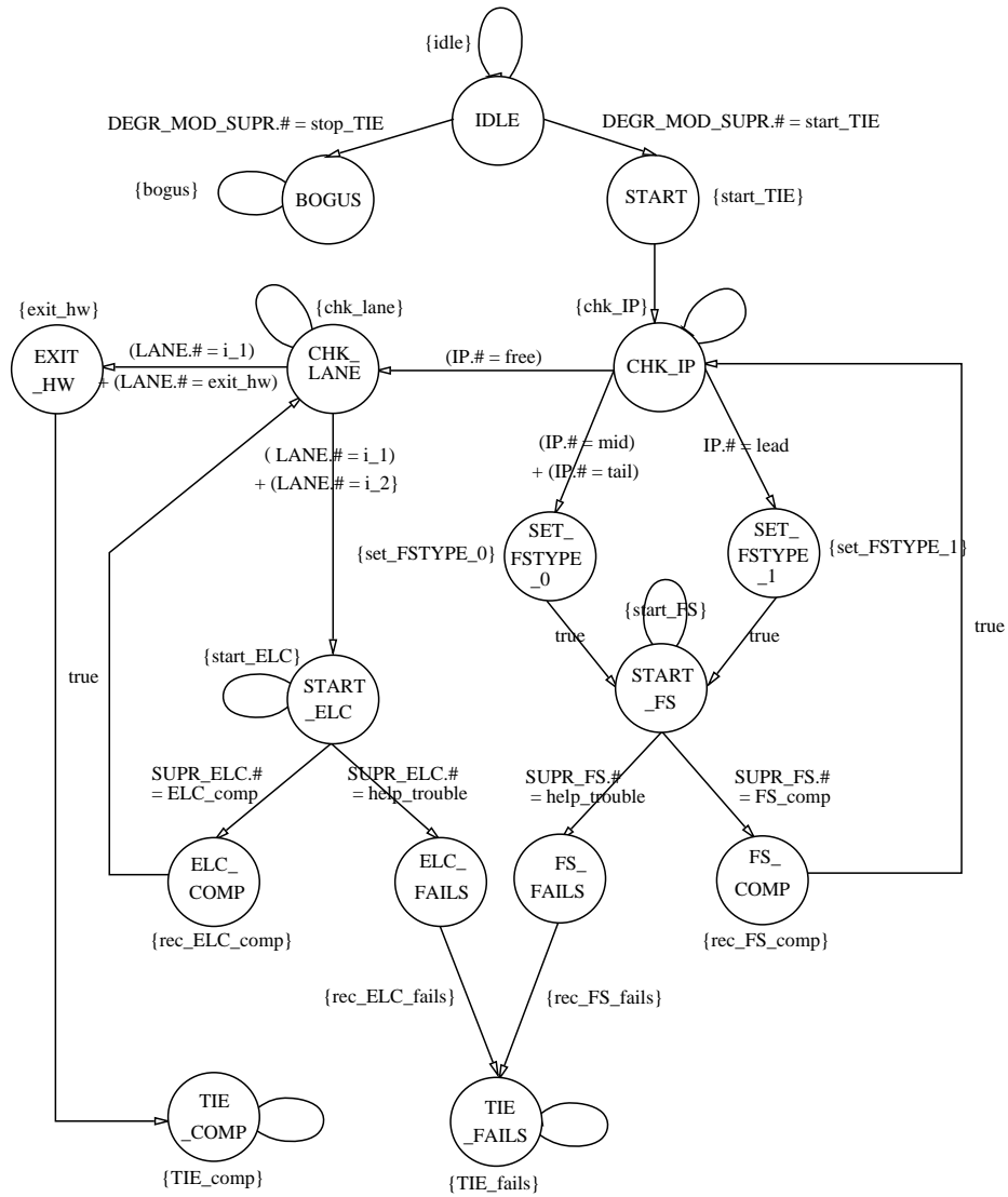
Figure 25: Take Immediate Exit Supervisor Processes
