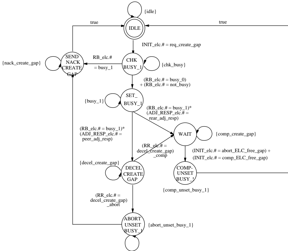
Figure 23: Emergency Lane Change Protocol Processes
