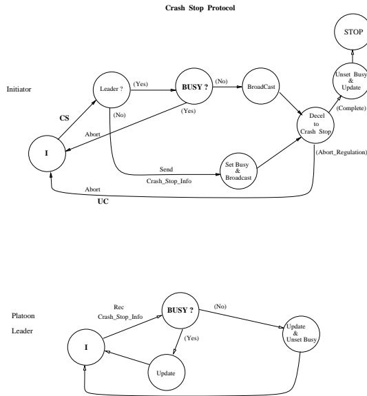
Figure 19: Crash Stop maneuver protocol
