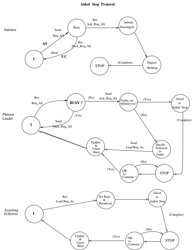
Figure 12: Aided Stop atomic maneuver protocol
