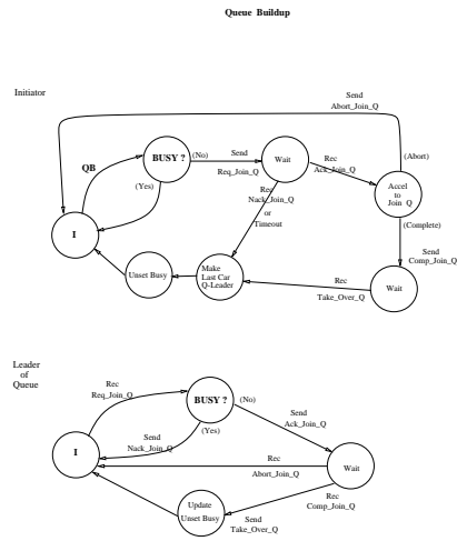
Figure 20: Queue Buildup
