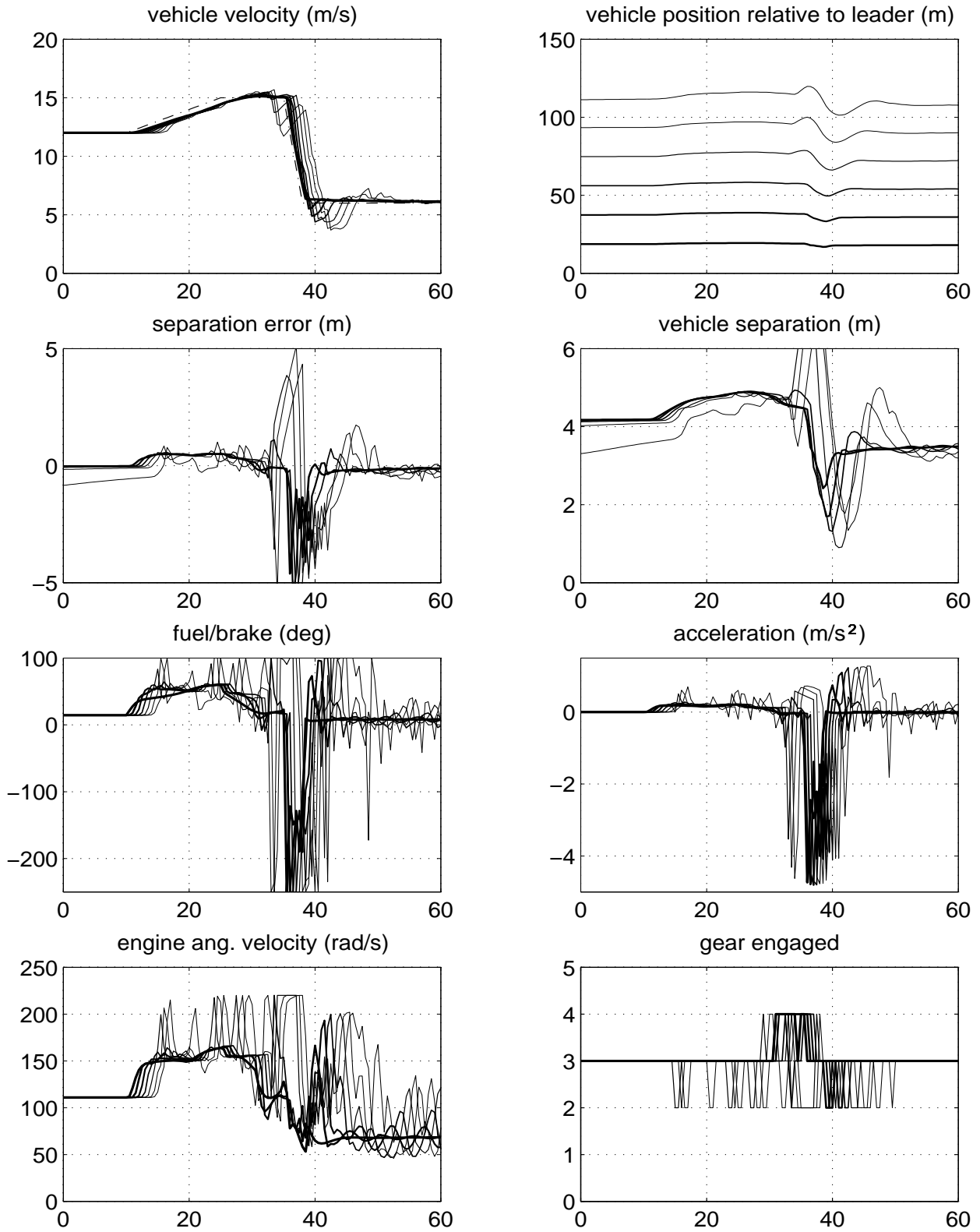
Figure 21: Actuator delay \tau = 0.3 s, backstepping controller, variable time headway h = 0.1 - 0.2v_r s, and variable separation error gain k = 0.1 + (1 - 0.1)e^{-0.1\delta^2} .
