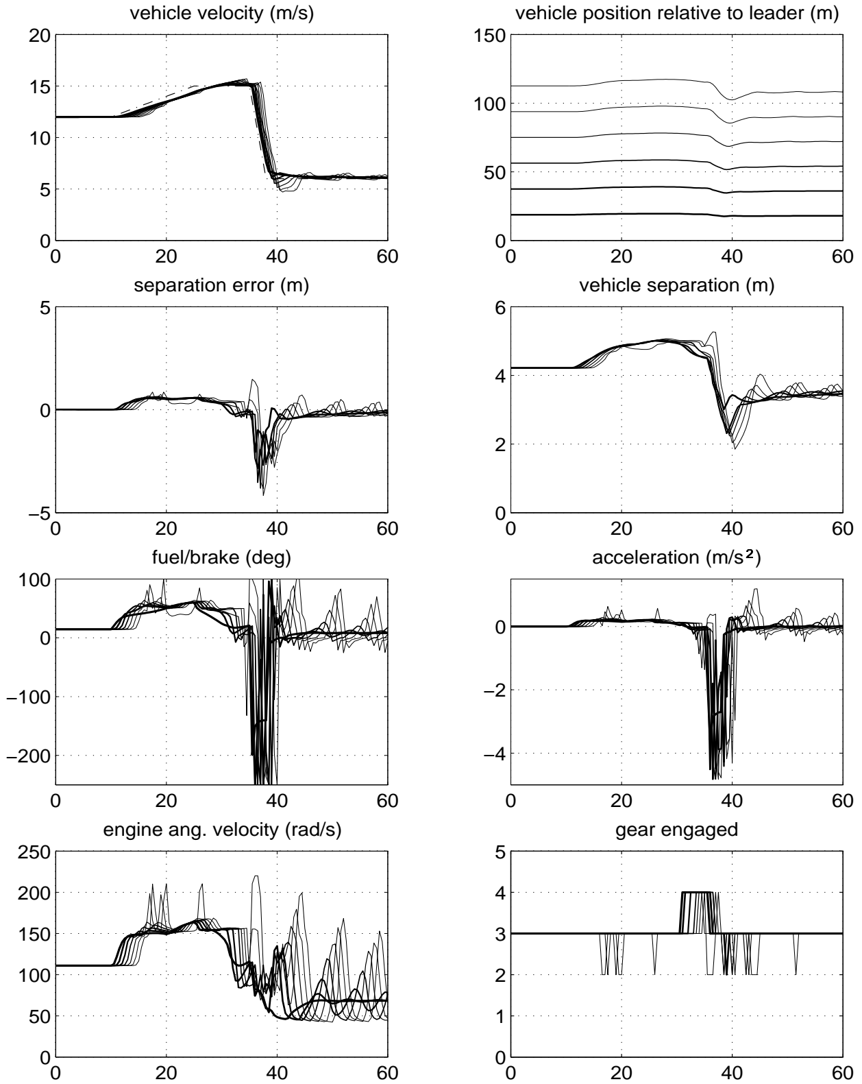
Figure 19: Actuator delay \tau = 0.2 s, backstepping controller with Smith predictor variable time headway h = 0.1 - 0.2v_r s, and variable separation error gain k = 0.1 + (1 - 0.1)e^{-0.1\delta^2} .
