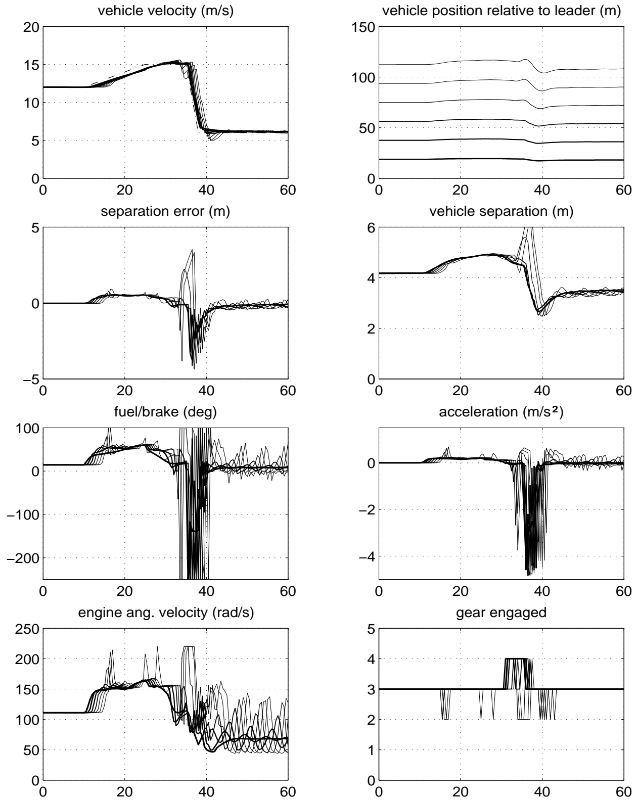
Figure 14: Actuator delay \tau = 0.2 s, backstepping controller with variable time headway h = 0.1 - 0.2v_r s and variable separation error gain k = 0.1 + (1 - 0.1)e^{-0.1\delta^2} .
