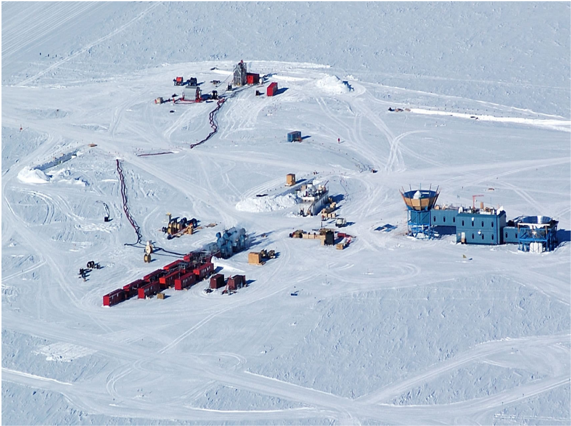
Figure 3.9: IceCube's 5 MW hot-water drill at work. In the lower left, a series of red trailers houses heaters and pumps. Hot water flows from these trailers through the black hose which snakes up to the tower structure in the upper center. This tower is situated over the hole which was being drilled at the time.
