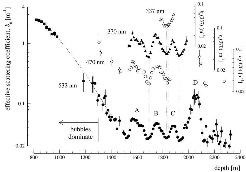
Figure 3.2: Scattering coefficient b_e as a function of depth below the surface of the icesheet. From [8].
