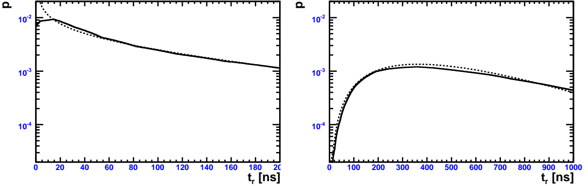
Figure 4.1: Pandel time residual pdf (dashed) compared to photonics [9] Monte Carlo simulation (solid) at distances of 25 m (left) and 125 m (right) from a cascade vertex located at a depth of 1948 m.
