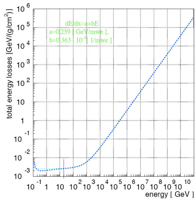
Figure 5.4: Total muon energy loss as a function of energy simulated by mmc. From [11].
