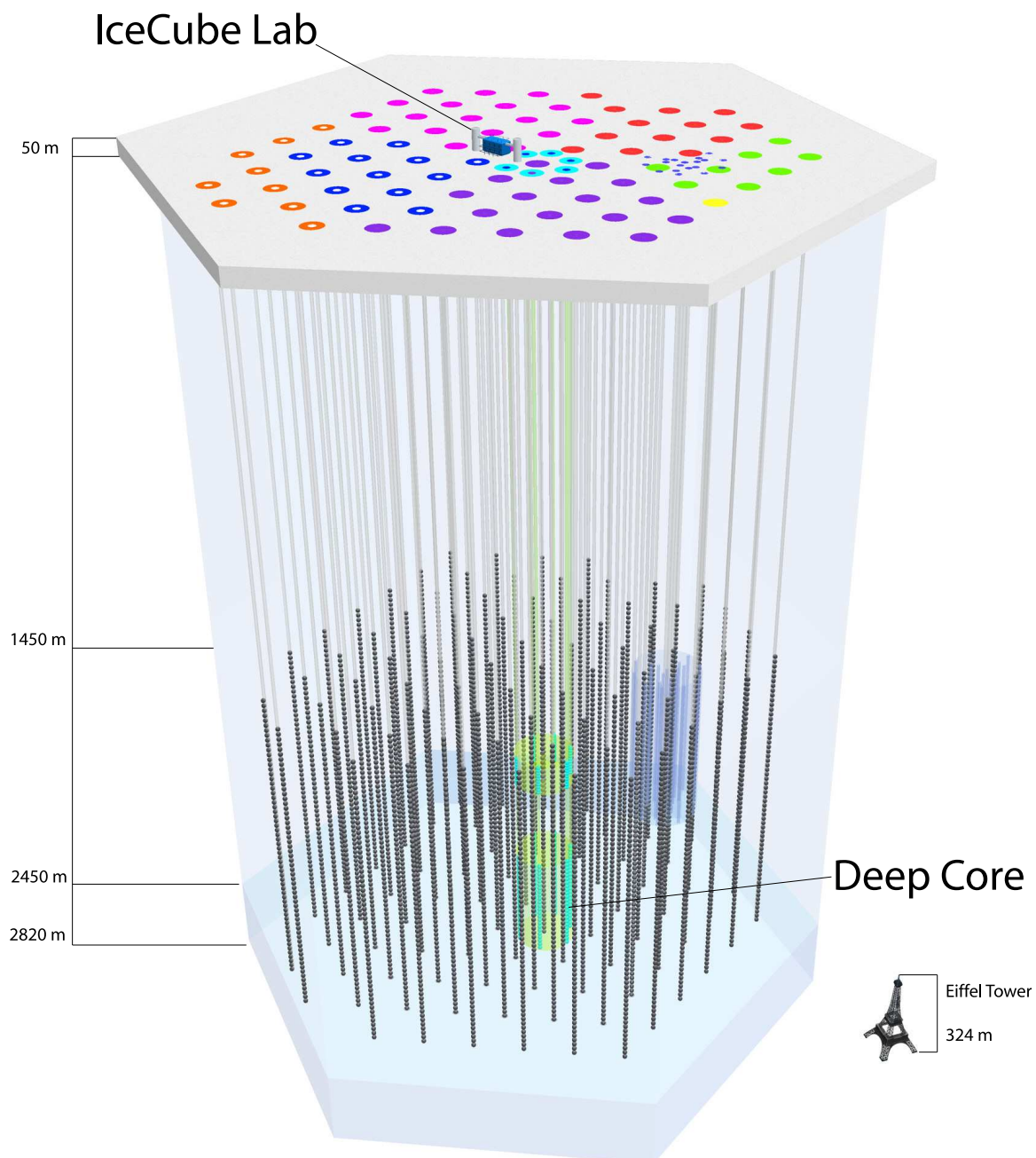
Figure 3.6: Schematic of the IceCube detector.
