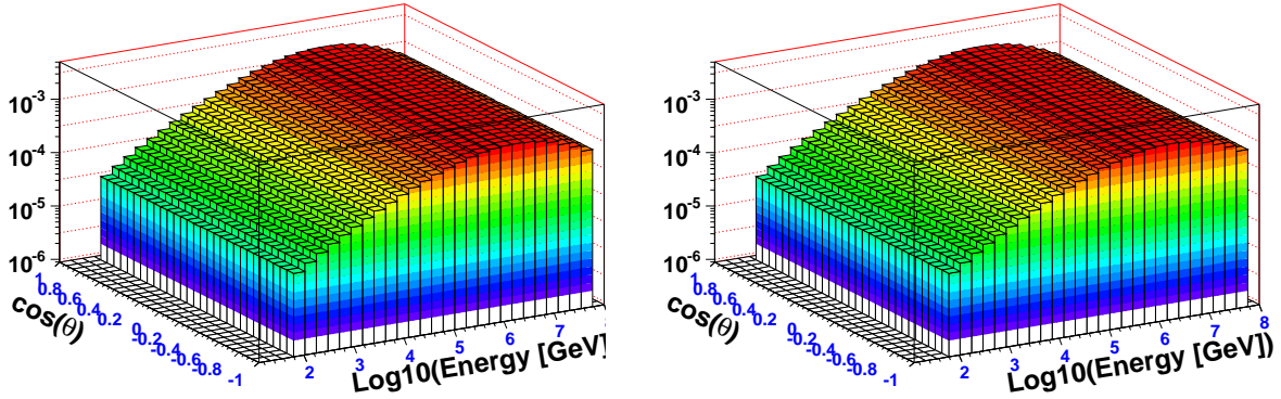
Figure 1.5: Prompt flux for muon neutrinos (left) and electron neutrinos (right) as a function of zenith and energy for the model from [3]. The fluxes have been multiplied by E^3 and have units of \text{GeV}^2 \text{cm}^{-2} \text{s}^{-1} \text{sr}^{-1} . The fluxes are isotropic.
