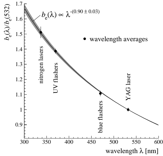
Figure 3.1: Wavelength dependence of the scattering coefficient b_e . From [8].
