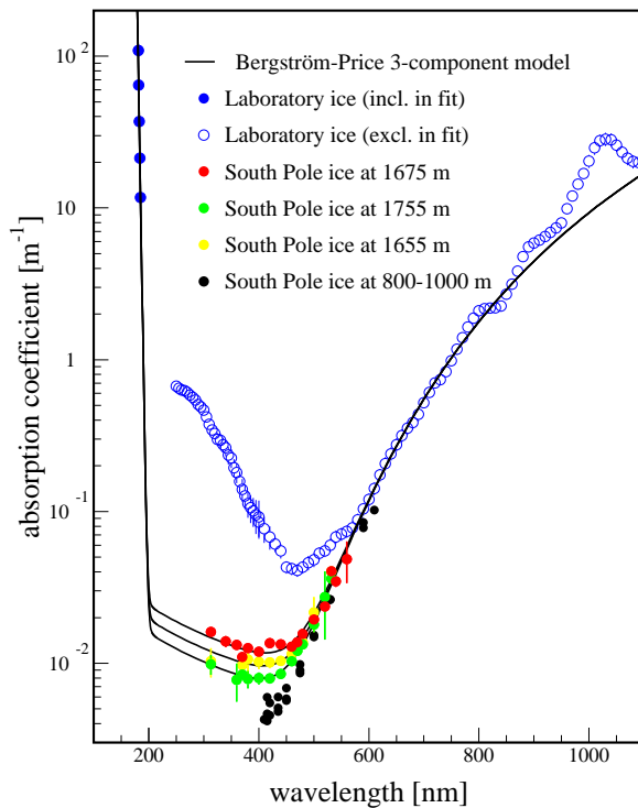
Figure 3.4: Wavelength dependence of the absorptivity a for glacial and laboratory ice. From [8].
