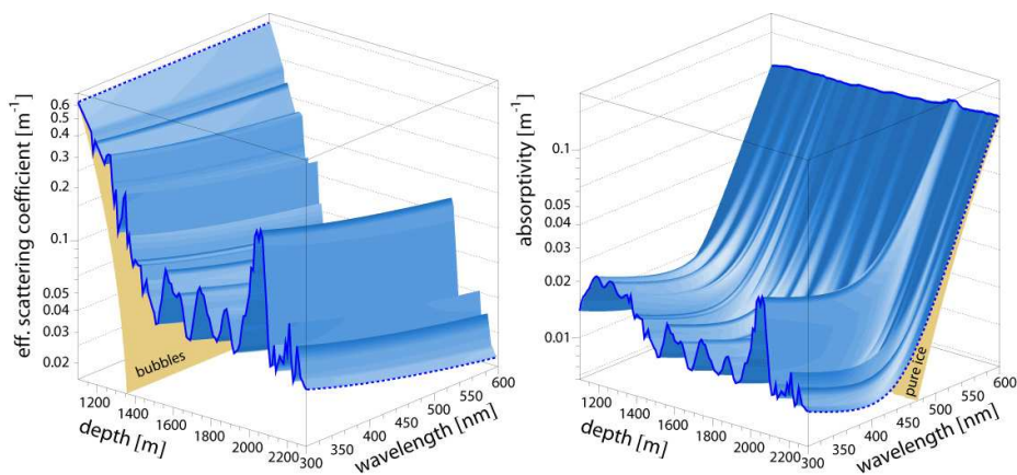
Figure 3.5: Scattering and absorption coefficients as a function of depth and wavelength. From [8].
