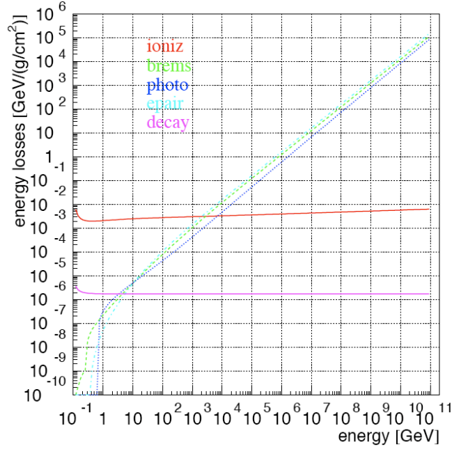
Figure 5.3: Muon energy loss processes simulated by mmc. From [11].
