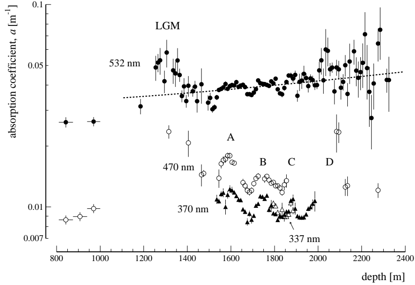
Figure 3.3: Absorption coefficient a as a function of depth below the surface of the icesheet. From [8].
