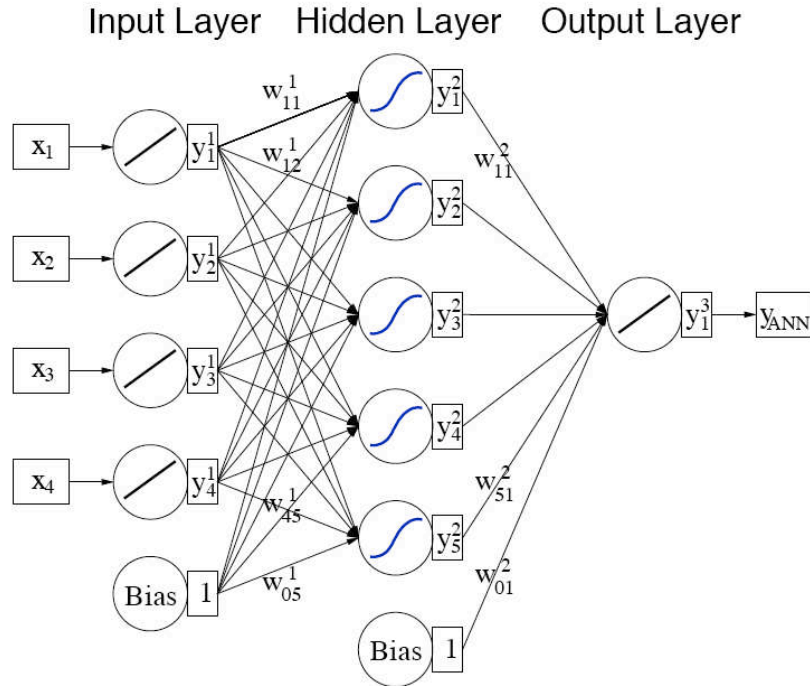
Figure 6.10: General layout of a multilayer perceptron (MLP). From [12].
