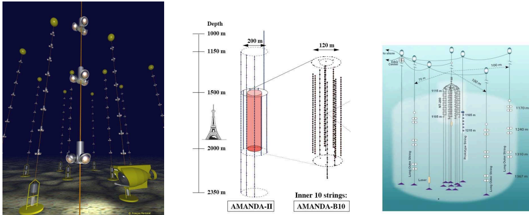
Figure 1.7: ANTARES (left, copyright F. Montanet, CNRS/IN2P3 and UJF for Antares), AMANDA (center, from [6]), and Baikal (right, from [7]).
