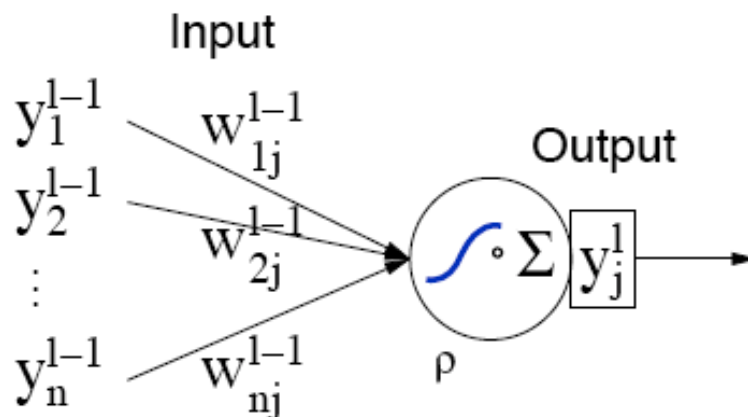
Figure 6.9: Schematic of a single neuron from a neural network. From [12].
