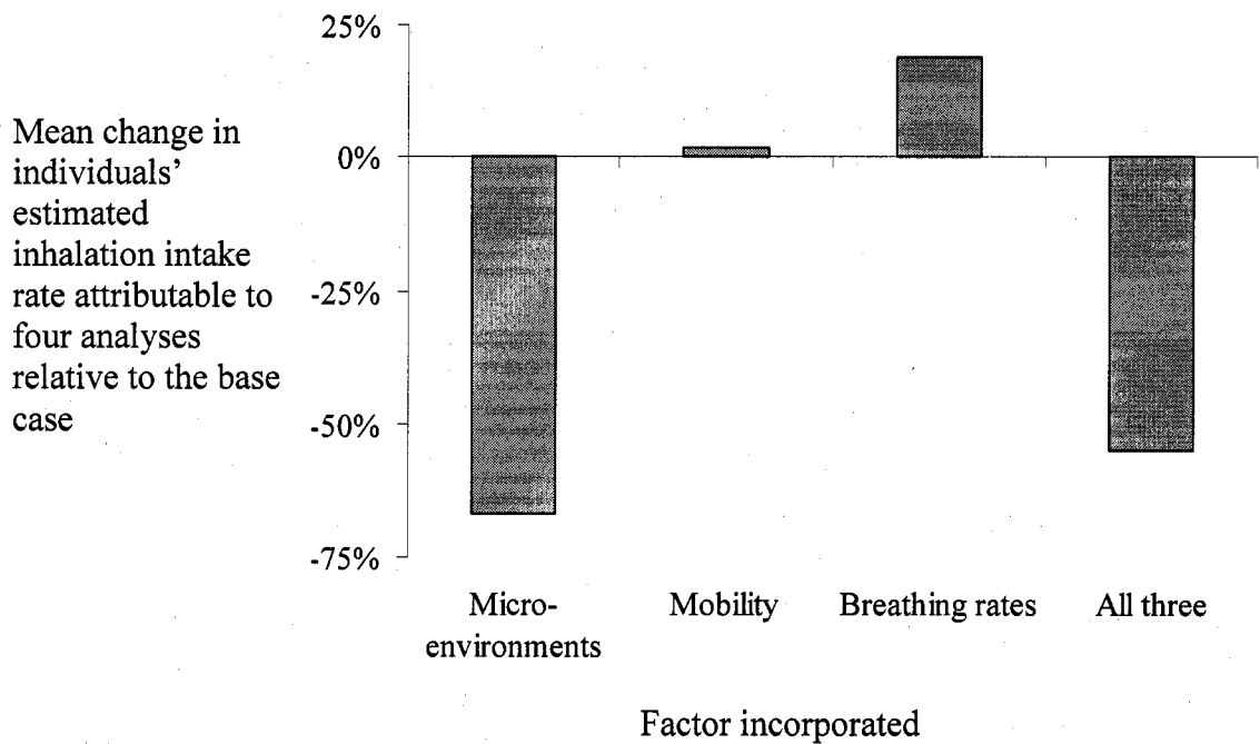
Figure 6-4e: ozone
