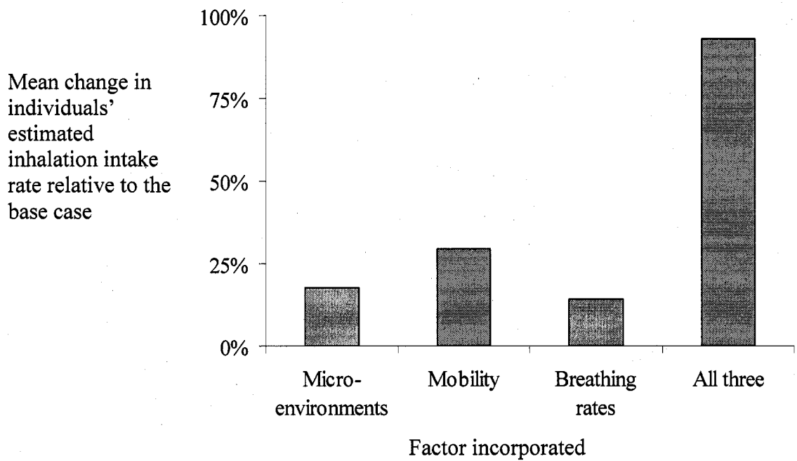
Figure 6-4b: 1,3-butadiene
