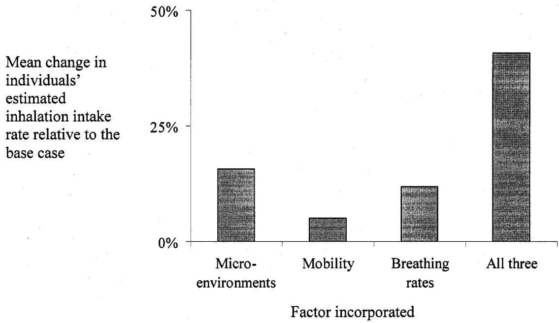
Figure 6-4a: benzene
