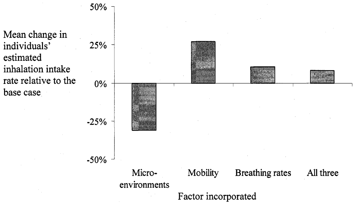
Figure 6-4c: diesel PM 2.5
