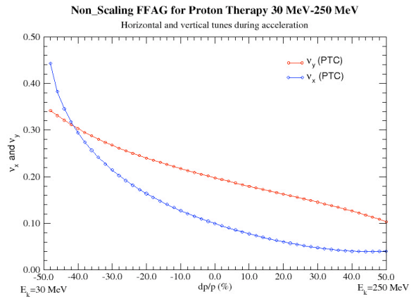
Figure 5. Horizontal and vertical betatron tune dependence on momentum.
