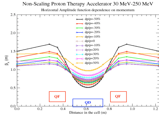
Figure 4. Horizontal amplitude \beta_x during acceleration.
