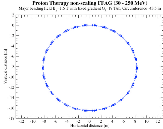
Figure 2. The whole ring of the fixed gradient lattice with 35 cells, C=43.5 m.
