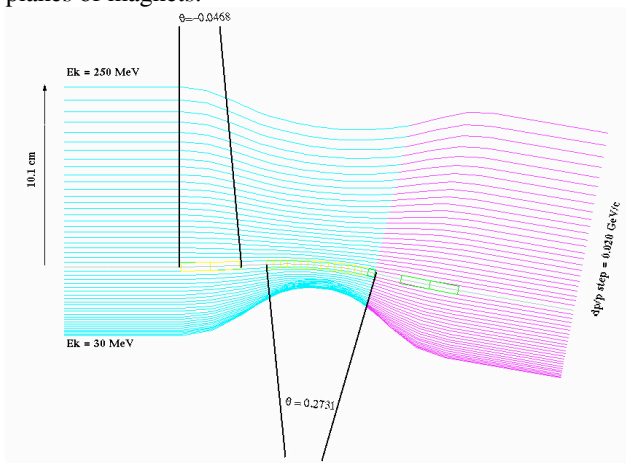
Figure 3. Orbits of particles during acceleration.
