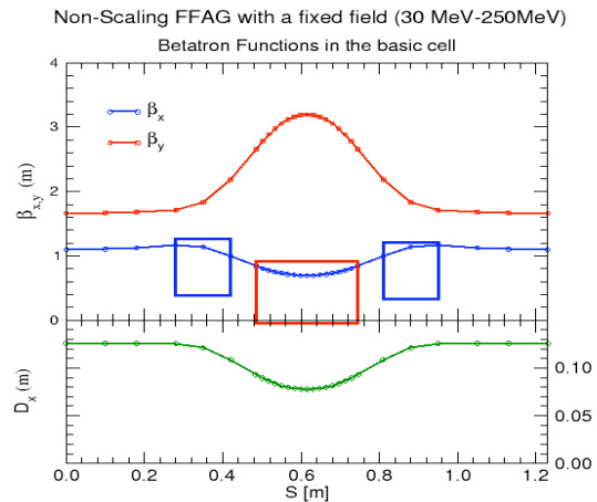
Figure 1. Betatron functions in the basic cell.
