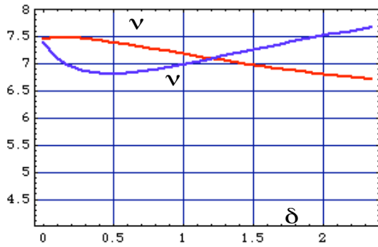
Figure 6. Horizontal and vertical tunes in the whole ring for the “Adjusted field profile” lattice.
