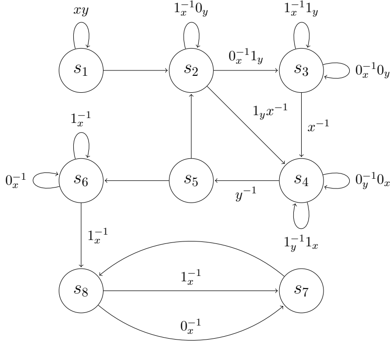
Figure 1.1: The graph \Gamma .
