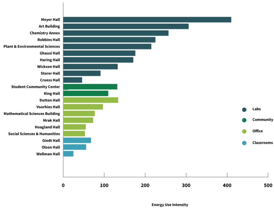
Figure 4. This energy visualization, referred to as Sorted Bar, is a bar chart representing EUI values, colored by building type, and sorted by both building type and EUI from highest to lowest.
