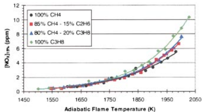
Fig. 11 \text{NO}_x concentrations for fully premixed cases
