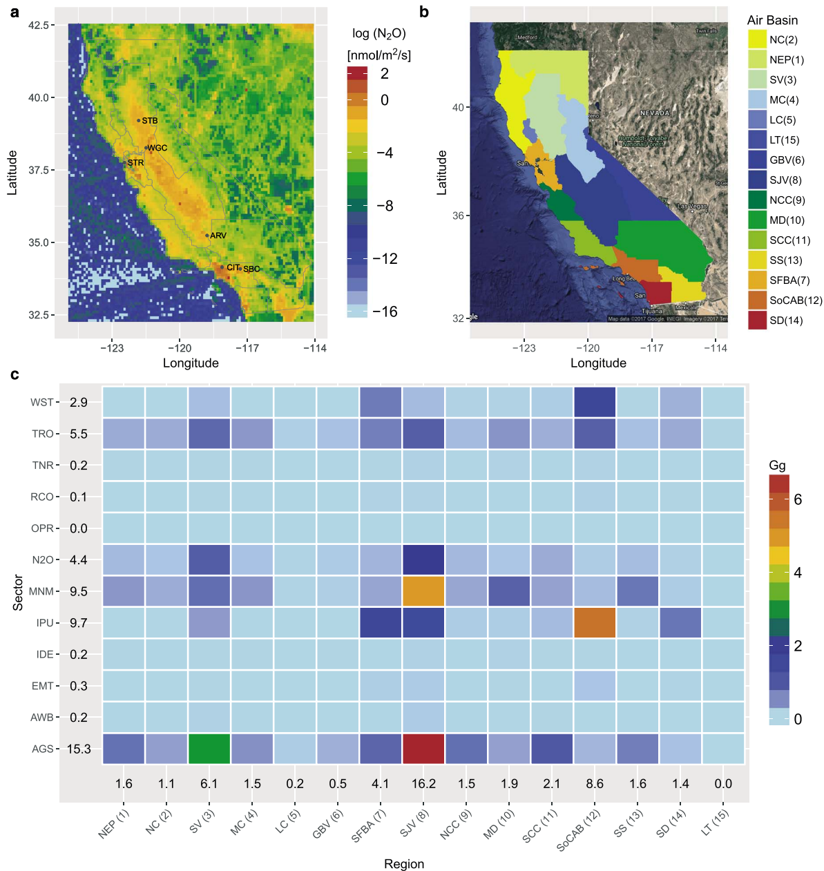
Figure 1. Prior N_2O emissions in California. (a) The total anthropogenic prior N_2O emissions used for inverse modeling (state total = 48.3 Gg N_2O /year) with locations of measurement sites across California, (b) region classification (California Air Basins, region numbers shown in the parentheses), and (c) emission summary ( Gg N_2O /year) by region and sector. In (c), sectors include agricultural soils (AGS), manure management (MNM), agricultural waste burning (AWB), industrial processes and product use (IPU), energy manufacturing transformation (EMT), indirect emissions from NO_x and NH_3 (IDE), indirect N_2O emissions from agriculture ( N_2O ), oil production and refineries (OPR), buildings (residential and others; RCO), waste (solid and wastewater; WST), nonroad transportation (TNR), and road transportation (TRO). Note that direct soil N_2O (AGS) is emitted from synthetic and manure fertilizers and crop residues left in the field while indirect N_2O emissions ( N_2O ) are from nitrogen leaching and runoff. The numbers on the left and bottom of (c) represent emission sums by sector and region, respectively.
