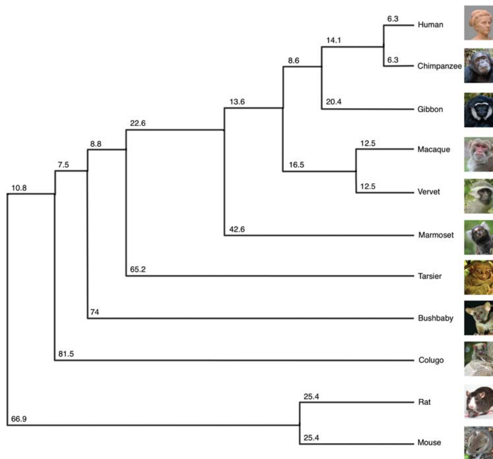
Figure 1. A phylogenetic tree depicting the position of vervet. The ultrametric tree with branch lengths is labeled in millions of years for the 11 mammalian species used in this study. Divergence times obtained from TimeTree ( www.timetree.org/ ).
