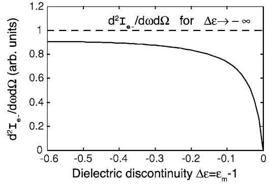
FIG. 2. The differential energy distribution d^2 I_e / d\omega d\Omega (solid curve) for an electron passing the dielectric discontinuity of the medium-vacuum interface ( \epsilon = \epsilon_m to \epsilon = 1 ), with \Delta\epsilon = \epsilon_m - 1 . The dashed line represents d^2 I_e / d\omega d\Omega in the (metal-vacuum) limit of \Delta\epsilon \rightarrow -\infty .
