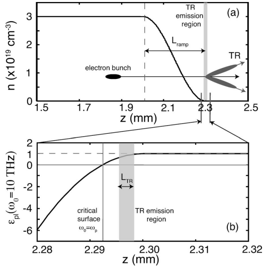
FIG. 1. (a) Longitudinal plasma density profile n(z) . (b) The spatially varying dielectric constant \epsilon_{pi}(z, \omega_0) for TR of frequency \omega_0 = 10 THz. The electron bunch is propagating from left to right.
