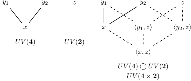
FIGURE 3. UV-sum of the UV-duals of the BAs \mathbf{4} and \mathbf{2} .
