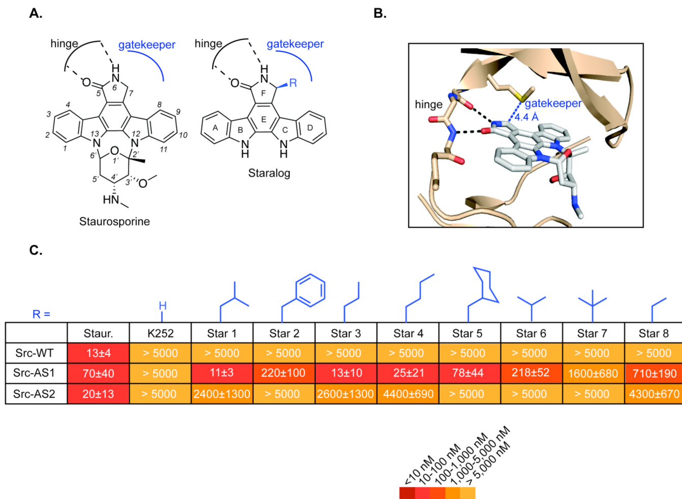
Figure 1. Design of staralog inhibitors and structure-activity relationships of the C7-position. (A) Structure of staurosporine (left) and engineered staralog inhibitors (right) with kinase hinge-binding interaction and gatekeeper pocket illustrated in black and blue, respectively. (B) X-ray co-crystal structure of staurosporine bound to Protein Kinase C \theta^{14} with hinge interaction highlighted in black and the distance between C7-position of staurosporine and the Met gatekeeper side chain highlighted in blue. (C) IC 50 values for staralog inhibitors against Src-WT, Src-AS1, and Src-AS2 kinases. IC 50 values were determined from a seven-point dose-response. Each experiment was done in triplicate and repeated for a minimum total of three times for compounds that showed measurable inhibition. Compounds that showed no inhibition were measured twice. Reported values represent the mean and error represents the standard error of the mean. WT = native gatekeeper (Thr for Src), AS1 = Gly gatekeeper, AS2 = Ala gatekeeper
