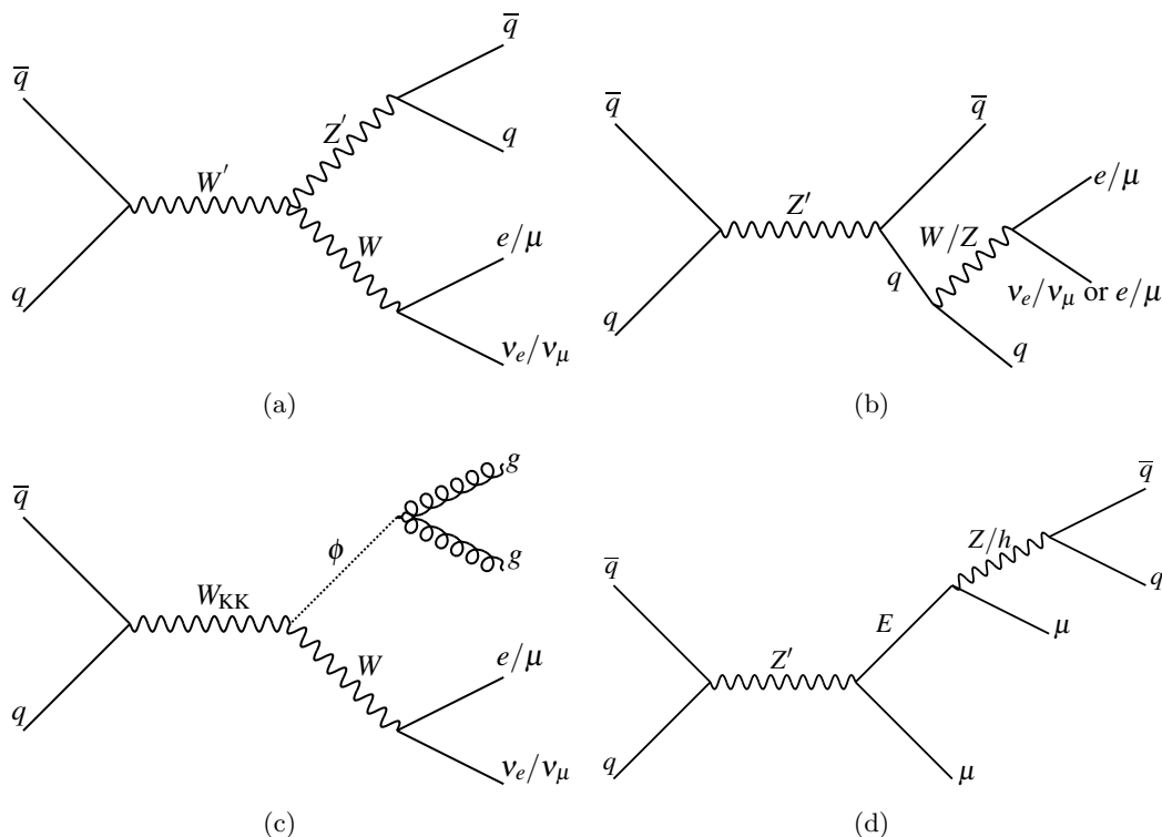
Figure 1. Representative Feynman diagrams for the models considered in this analysis: (a) W' \rightarrow Z'W production in the SSM, (b) the simplified DM model, (c) the radion model, (d) the composite-lepton model. The text provides more detailed descriptions.
