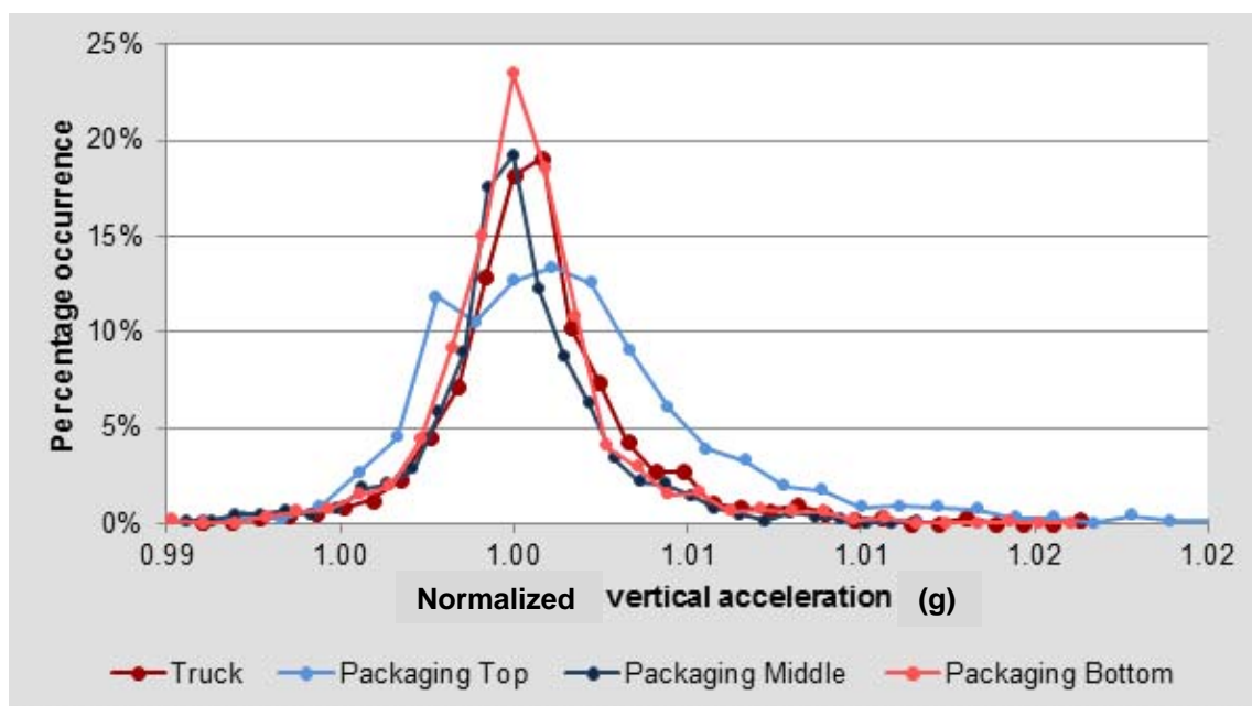
Figure 5.13: Normalized distributions of the vertical accelerations experienced within pallets at various packing levels at the front of the truck.
