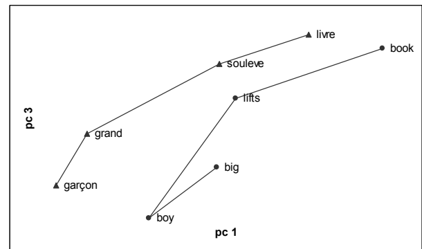
Figure 5: Trajectories in state space (factor plane 1x3) for big boy lifts book and garçon grand souleve livre .
