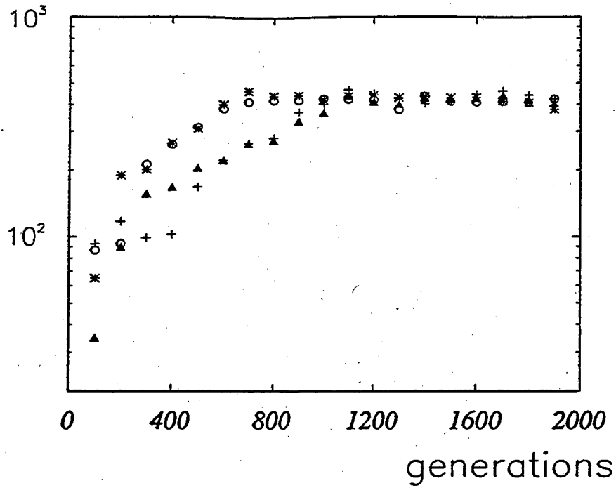
Figure 3: Number of synapses (5 Bit parity)
