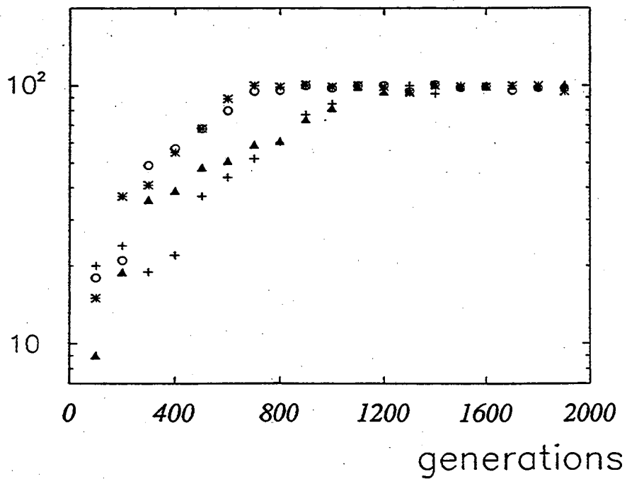
Figure 2: Number of neurons (5 Bit parity)
