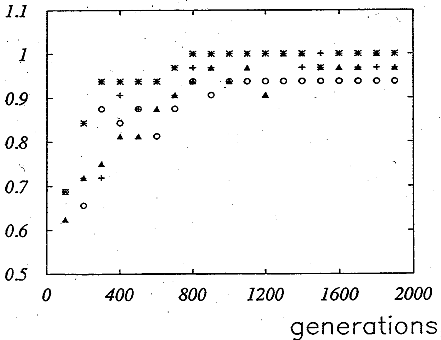
Figure 4: Fraction of correct Bits (5 Bit parity)
