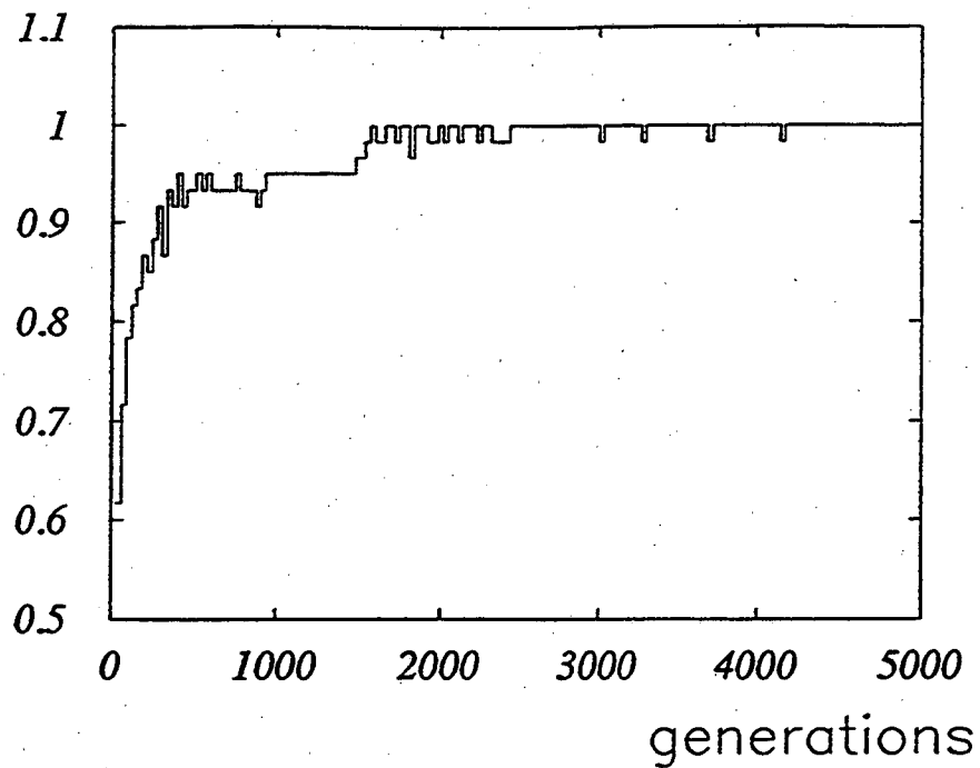
Figure 7: Fraction of correct Bits (Counting problem)
