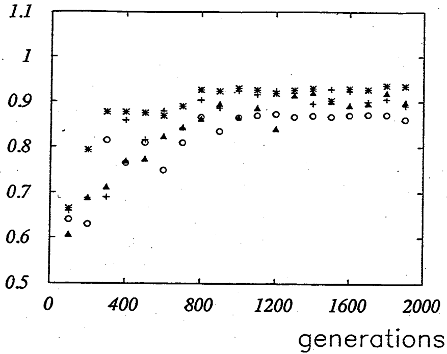
Figure 1: Fitness (5 Bit parity)
