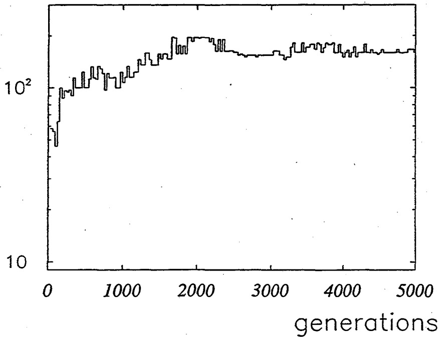
Figure 10: Number of synapses (Counting problem)
