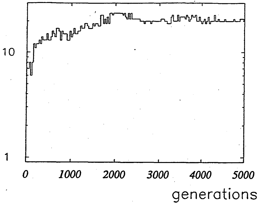
Figure 9: Average cortex size (Counting problem)
