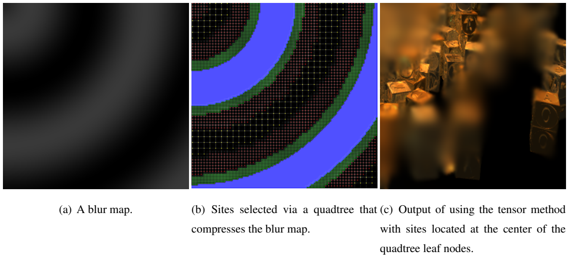
Figure 7.5: Illustration of the tensor method with a quadtree used to lay out the sites.
