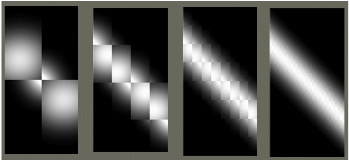
Figure 7.1: Using the SVD to find the best separable approximation of blocks within the matrix. From left right, the blocks are of increasingly small size.
