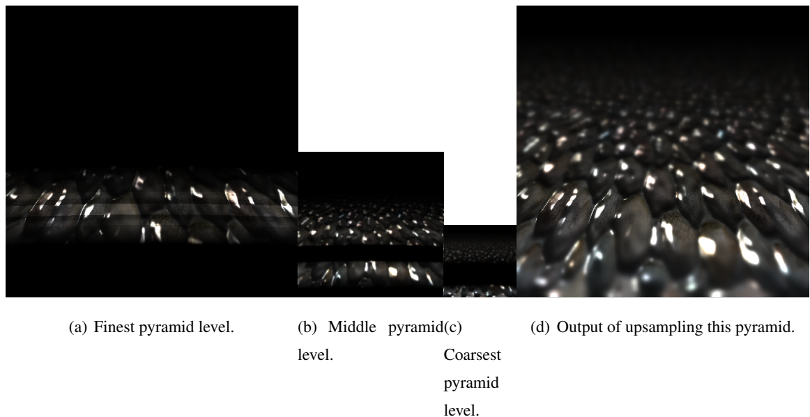
Figure 6.8: The pyramid method spreads PSFs to various pyramid levels, then upsamples the levels through the pyramid to yield a final, blurred image.
