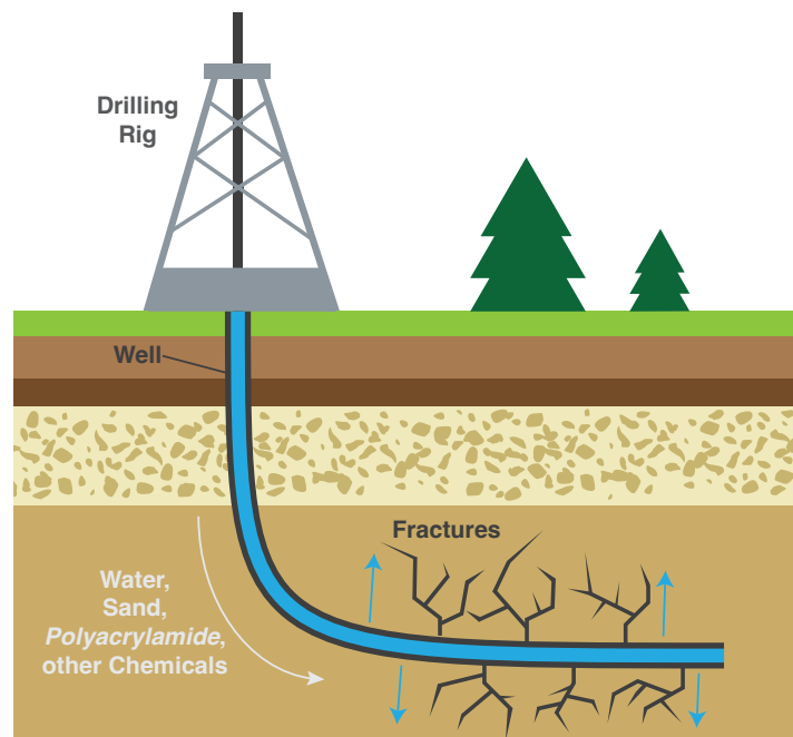
Figure 4.1 Schematic representation of hydraulic fracturing. Water, sand, friction reducers, and other chemicals are pumped into oil or gas rich layers of earth to create and maintain fractures.
