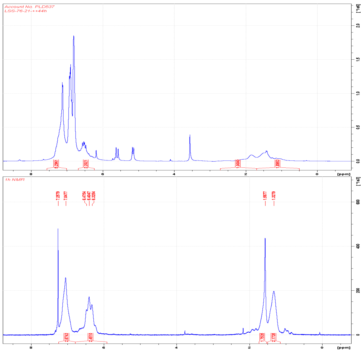
Figure S25. ^1\text{H} NMR (300 MHz, 25^\circ\text{C} ) spectra of PCS-PS-PCS copolymerization reaction after adding p-CS again in \text{C}_6\text{D}_6 (top) and the isolated polymer of PCS-PS-PCS in \text{CDCl}_3 (bottom, Table 2, entry 5). \delta (ppm): 7.05 (m, 2H, ArH, PS and PCS), 6.33 (m, 2H, ArH, PCS), 1.57 (br t, 1H, \text{CHCH}_2 , PS and PCS), 1.33 (br d, 2H, \text{CHCH}_2 , PS and PCS).
