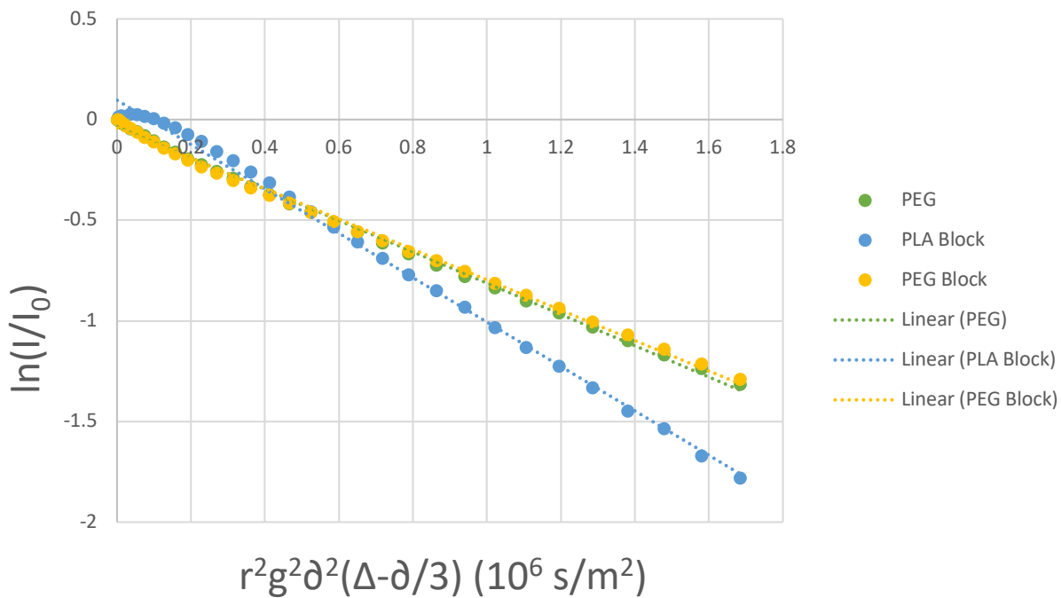
Figure S60. Stejskal-Tanner plot of the diffusion activity of the PEG and PLA in the product of the PEG quenching experiment.
