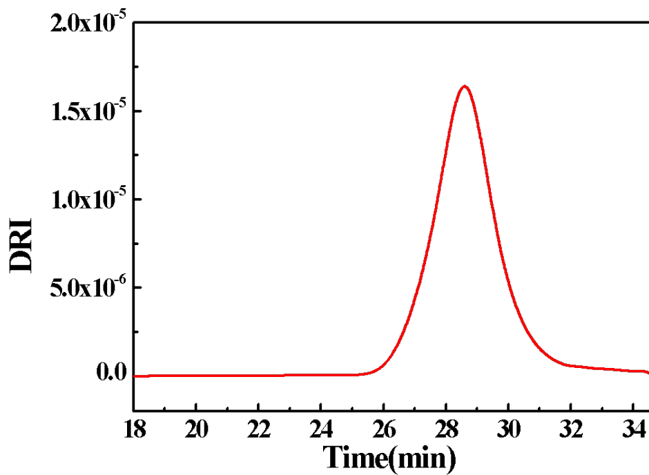
Figure S37. SEC trace of PCS homopolymer using (fc^{P,B})NiBr at 25°C (Table 2, entry 3).
