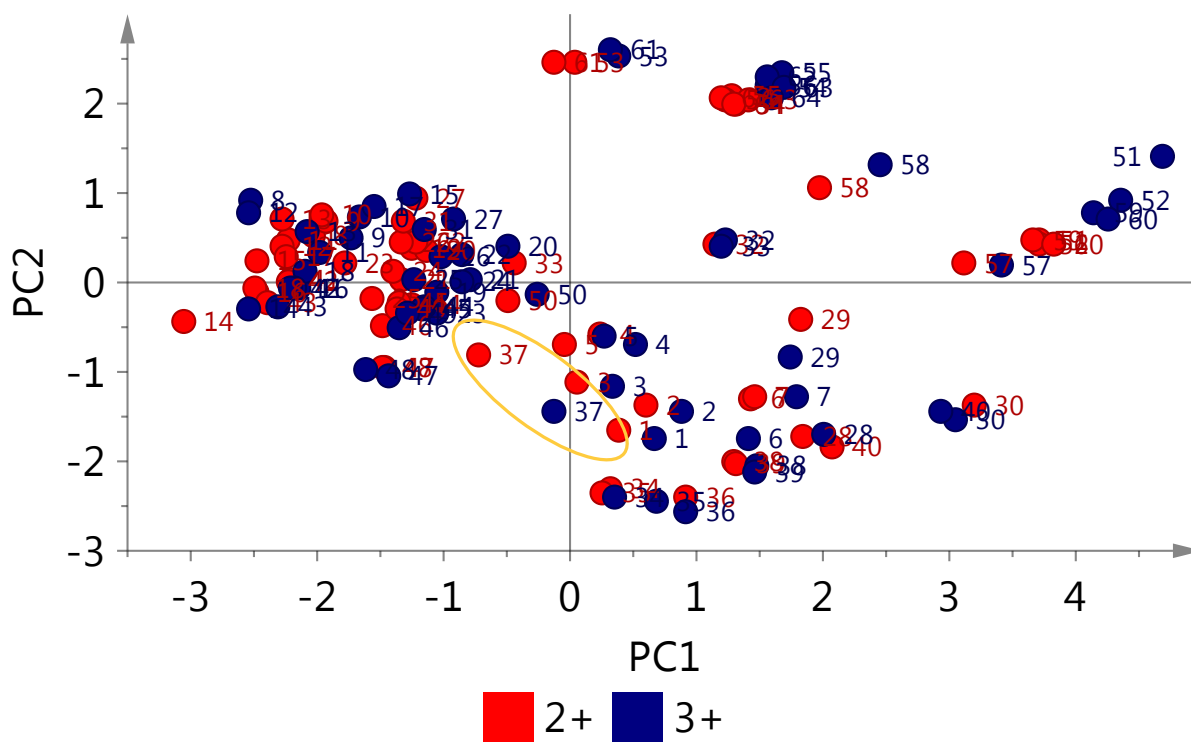
Figure 3.2 PCA plot for various ferrocene-based ligand frameworks coordinating different metals treating each oxidation state as a different entry oxidation states of ferrocene. The circled 37 is the (salen)Sc compound at the focus of this chapter. Reprinted with minor modifications from Lai, A.; Clifton, J.; Diaconescu, P. L.; Fey, N. Computational mapping of redox-switchable metal complexes based on ferrocene derivatives. Chem. Commun. 2019 , 55 (49), 7021-7024, with permission from the Royal Society of Chemistry.
