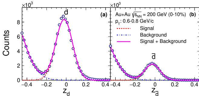
FIG. 2. The z(d) distributions for positively (a) and negatively (b) charged particles in the TPC at p_T = 0.6 - 0.8 GeV/c in 0 – 10% centrality Au+Au collisions at \sqrt{s_{NN}} = 200 GeV. The curves are two-Gaussian fits for signal and background. Uncertainties are statistical only and are smaller than the marker size.
