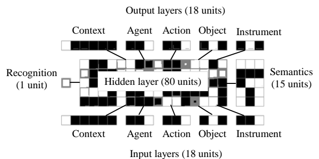
Figure 1: The architecture of the model (Hinton diagram).
