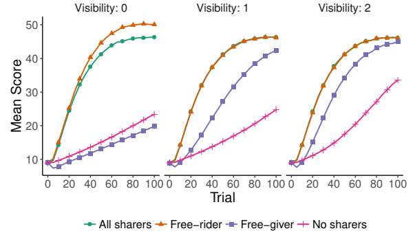
Figure 2: Learning curves. Mean score for 10,000 replications using k = 10 agents and n = 7 dimensions, and with innovation rate p_c = 0.5 . Each line is either a random agent drawn from the all sharers or no sharers condition, or specifically the heterodox agent in the free-rider and free-giver conditions. Across different visibility radii, we see how the maladaptiveness of sharing (left panel) disappears, and transforms into an adaptive benefit. With a visibility of 1, the benefits of free-riding are reduced to zero, while the reversal for free-giving is much more dramatic and confers much larger rewards than the counter-factual case of withholding information (i.e., no sharer).
