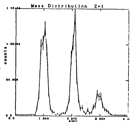
Fig. 27. Mass distribution z = 1 .
