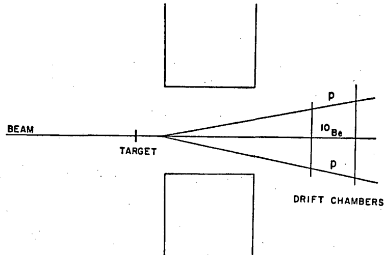
Fig. 3. Decay of a long-lived state.
