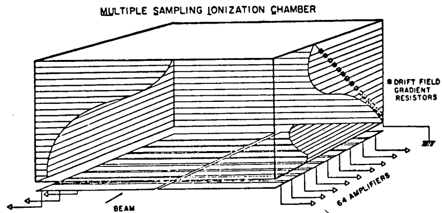
Fig. 13. MUSIC detector configuration.
