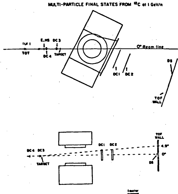
Fig. 23. HISS group experimental setup.
