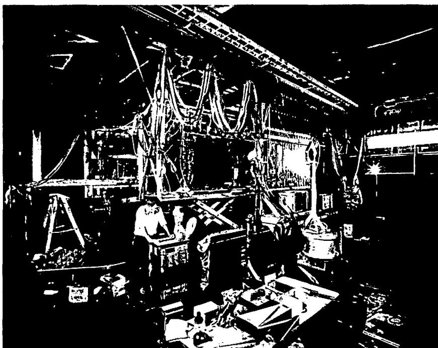
Fig. 10. Magnet vacuum tank and phase 1 drift chambers.
