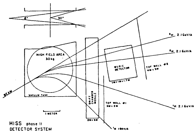
Fig. 7. Phase 2 instrumentation.
