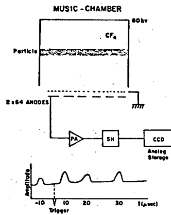
Fig. 15. MUSIC signal processing.
