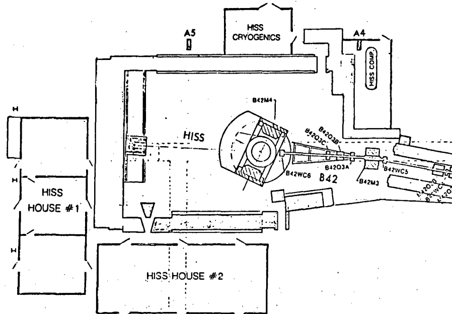
Fig. 5. HISS facility.
