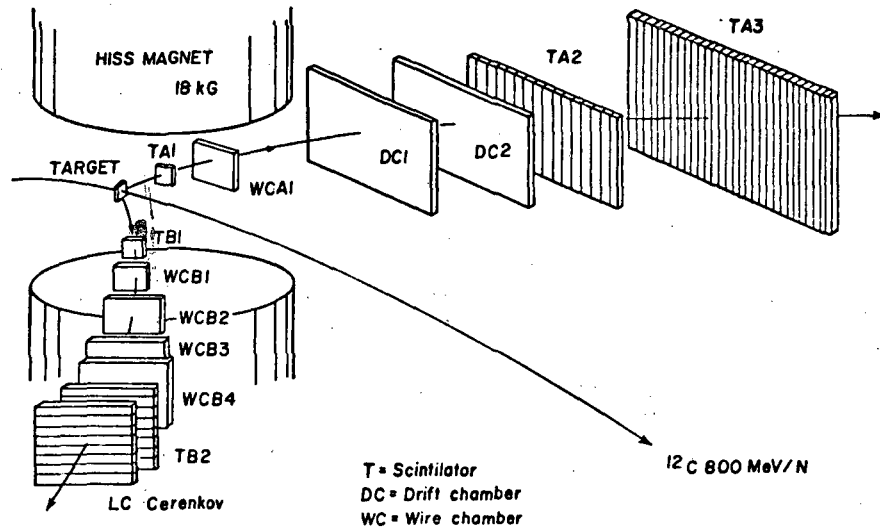
Fig. 20. INS experimental setup.
