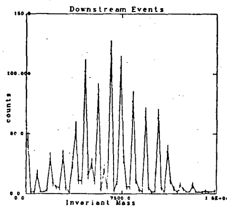
Fig. 33. Invariant mass distribution for downstream event sample.
