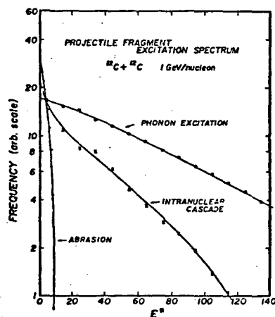
Fig. 2. Predicted interaction energy spectrum.
