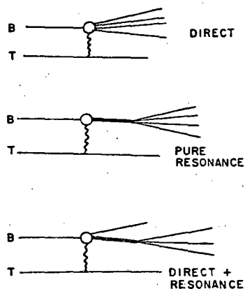
Fig. 1. Some possible reaction sequences.
