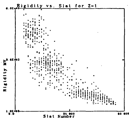
Fig. 26. Rigidity versus TOF slat number, z = 1 .
