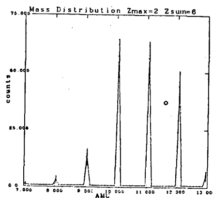
Fig. 29. Mass distribution for events with maximum charge = 2 and charge sum = 6.
