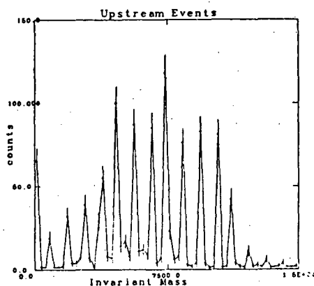
Fig. 32. Invariant mass distribution for upstream event sample.
