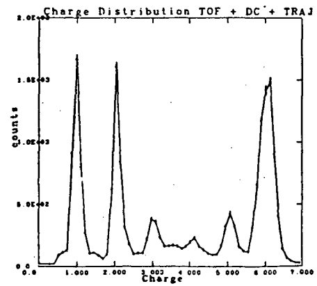
Fig. 25. Charge distribution TOF + drift chamber trajectory.
