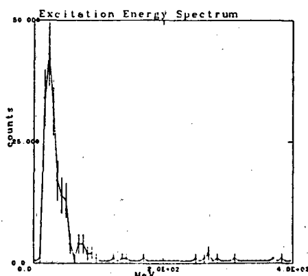
Fig. 30. Excitation energy spectrum.
