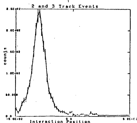
Fig. 31. 2 and 3 track interaction positions.
