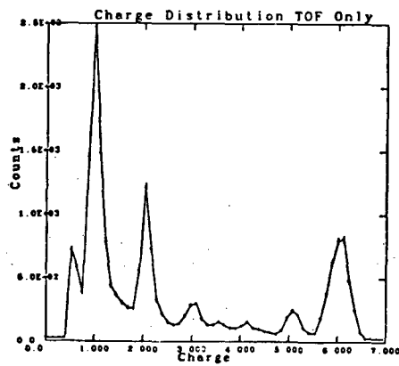
Fig. 24. Charge distribution in TOF wall.
