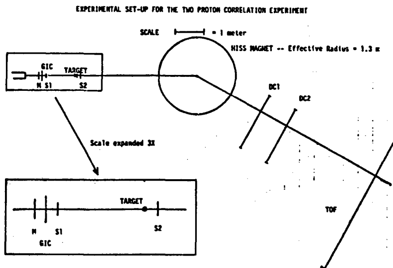
Fig. 22. Igo et al. experimental setup.
