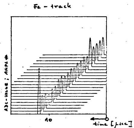
Fig. 16. MUSIC response to ^{56}\text{Fe} beam.
