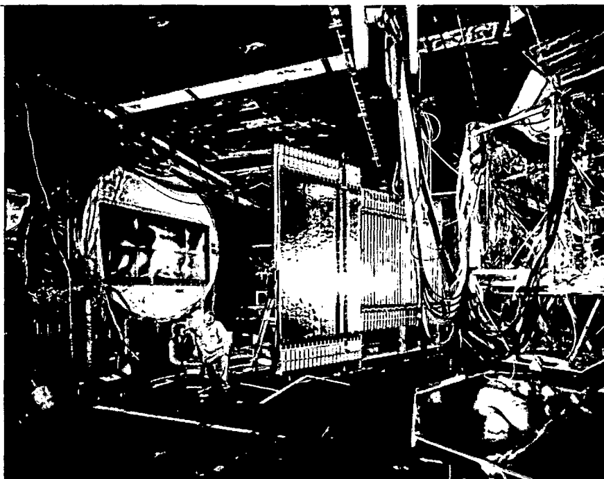
Fig. 9. HISS cave with TOF walls and MUSIC detector.
