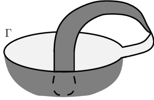
A pseudo-area minimizing disk is embedded everywhere except where \Gamma meet interior.
