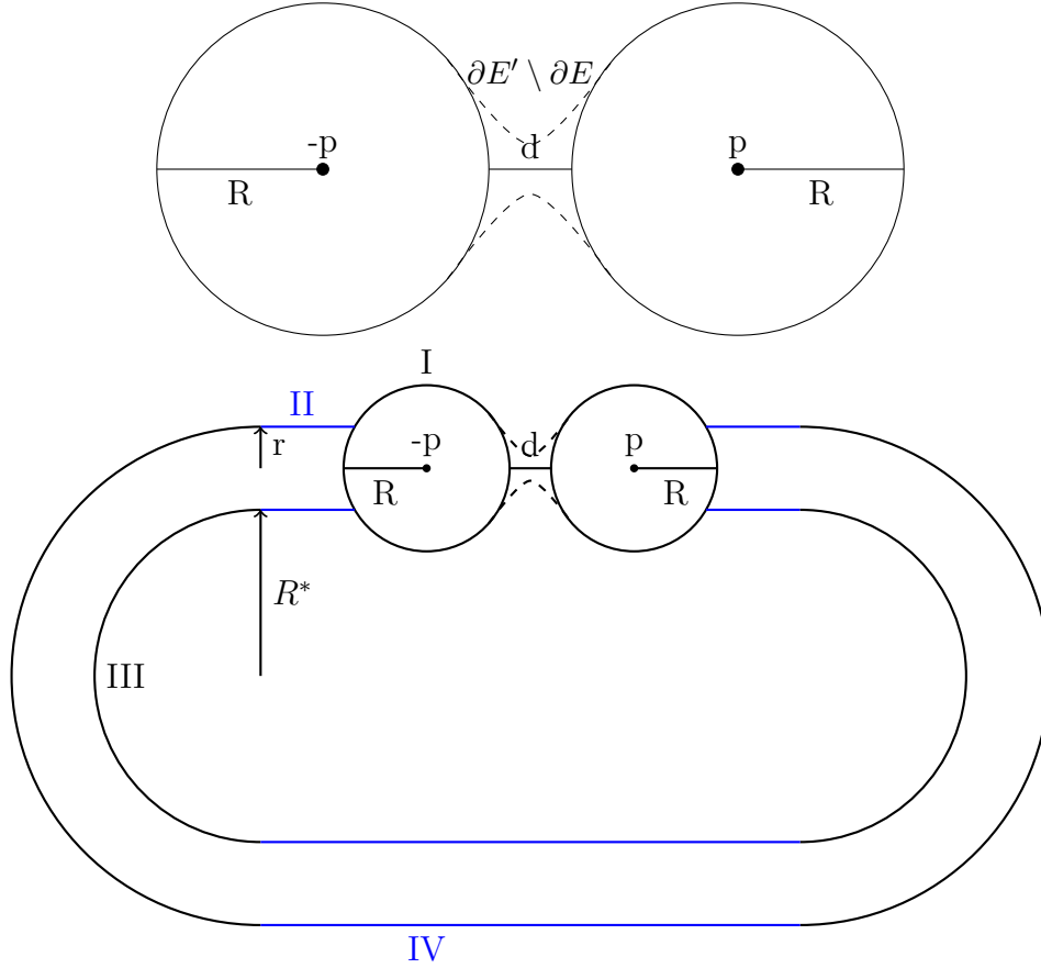
FIGURE 2.2. Given sufficiently close disjoint balls, one can attach handles and glue them together so that the resulting C^2, H > 0 surface is not strictly outward minimizing.
