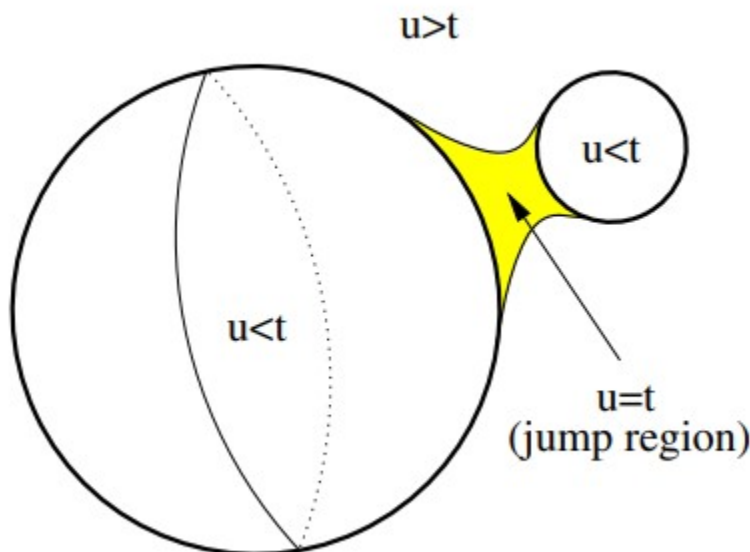
FIGURE 1.3. Two spheres evolved by the classical flow will eventually cease to be strictly outward-minimizing by the time t , triggering a jump across the region \{u = t\} in the weak flow. Image from page 374 of [HI01].
