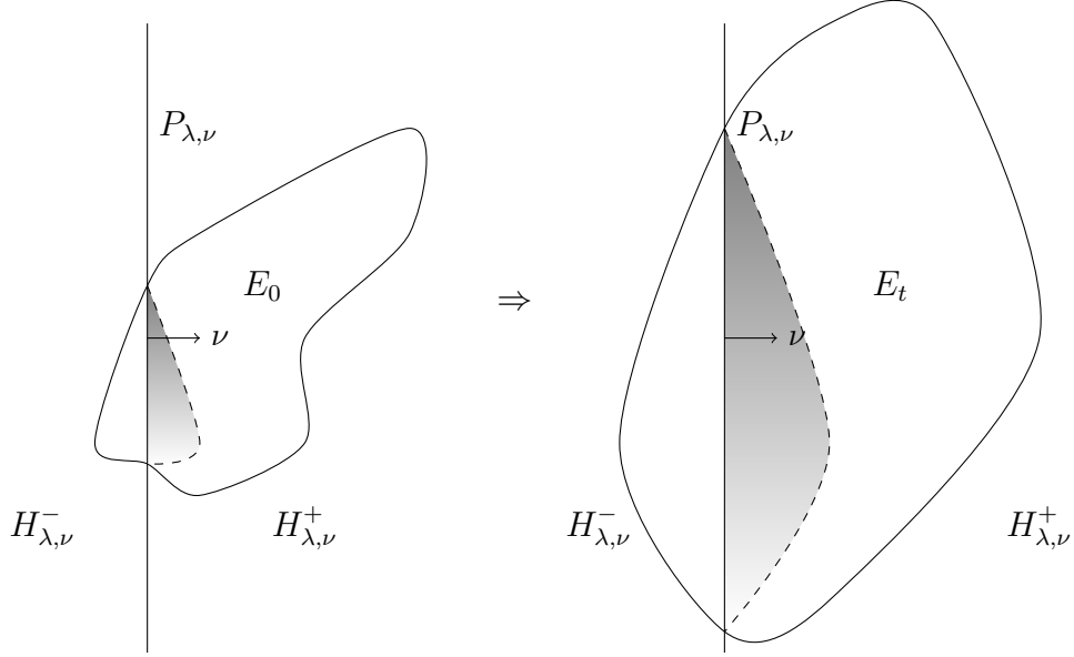
FIGURE 2.1. Given a set E_0 which is initially admissible with respect to some plane, the corresponding solution \{E_t\}_{0 \leq t \leq T} to weak IMCF remains admissible for every t .
