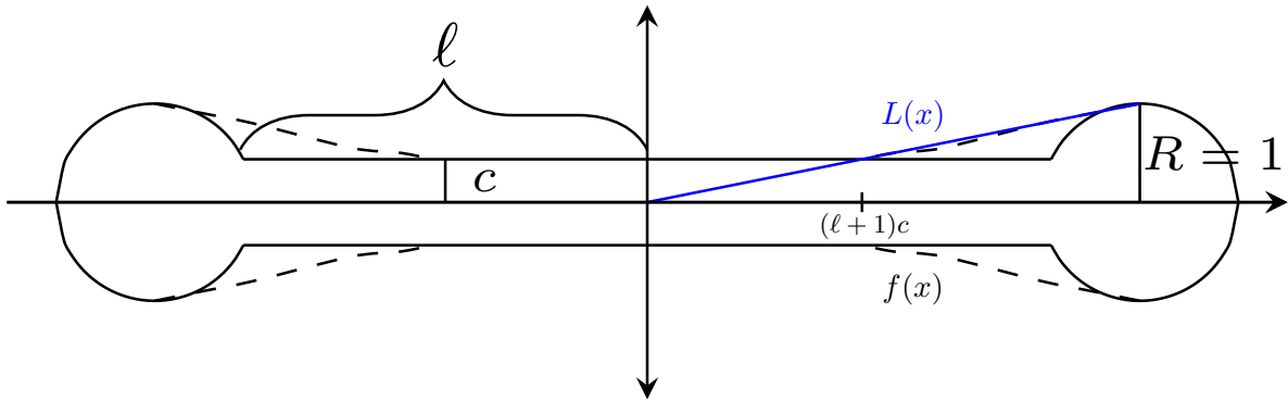
FIGURE B.1. Smoothing spheres attached to a sufficiently long neck produces a non-star-shaped, admissible surface of revolution.
