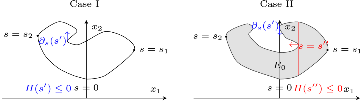
FIGURE 3.1. If \langle e_2, \nu \rangle = 0 at some point between s_1 and s_2 , one can locate a point where \langle e_2, \nu \rangle = 0 and k \leq 0 .
