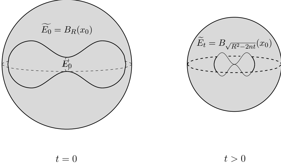
FIGURE 1.1. Comparison of a closed solution of MCF with a sufficiently large sphere establishes the existence of a finite-time singularity.
