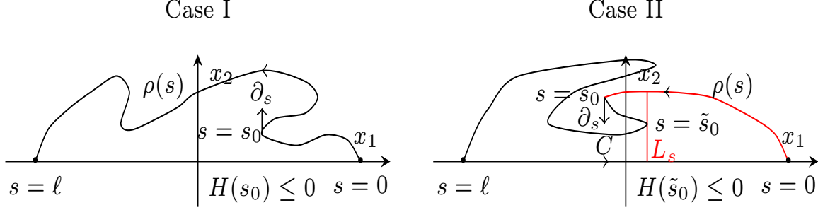
FIGURE 4.2. If \langle e_2, \nu \rangle = 0 at some interior point of \rho , one can locate a point where \langle e_2, \nu \rangle = 0 and k \leq 0 .
