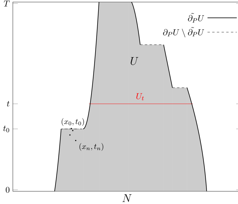
FIGURE 4.4. For a non-cylindrical domain U \subset N \times [0, T) , the reduced parabolic boundary \tilde{\partial}_P U does not include the dotted parts of \partial_P U . If every point in \partial_P U \setminus \tilde{\partial}_P U can be approached in U from below in time, \sup_U f cannot occur at any of these points.
