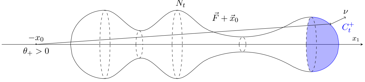
FIGURE 4.5. By picking a point on the axis away from the flow surfaces for t \in [0, T) , we ensure the support function is positive over the right cap.
