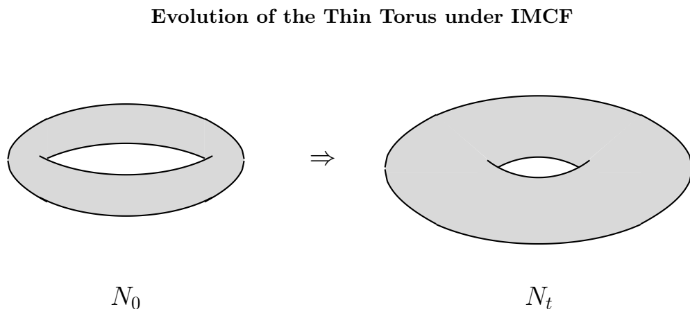
FIGURE 1.2. The thin torus evolved by IMCF will continue to expand until the flow speed along the inner ring becomes infinitely large.
