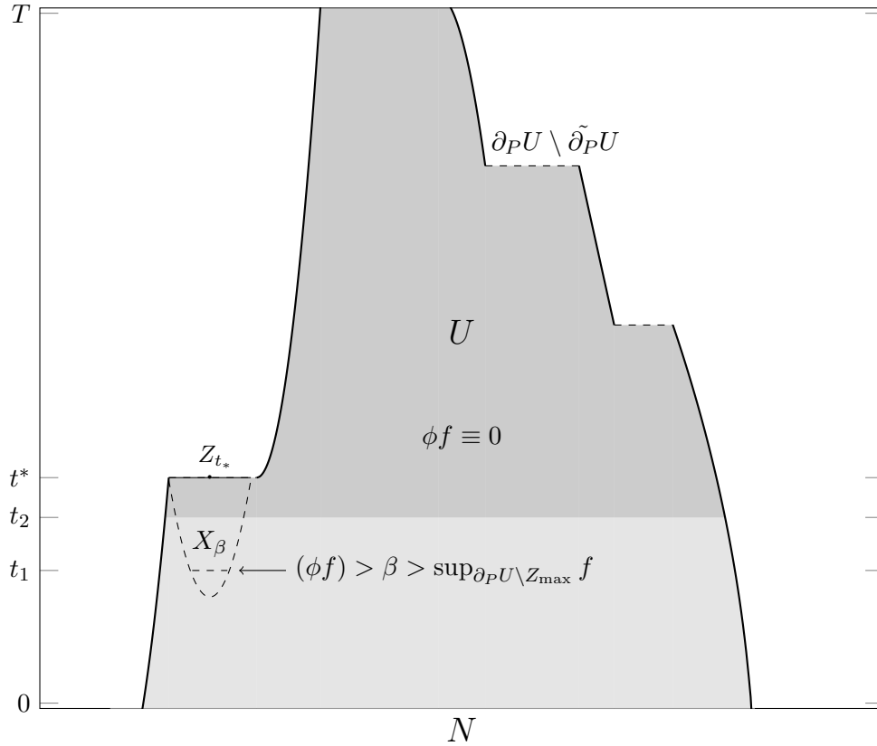
FIGURE A.1. The cutoff function \phi is 1 for times less than t_1 and 0 for times greater than t_2 . This guarantees that the supremum of \phi f occurs at an interior point of X'_\beta .
