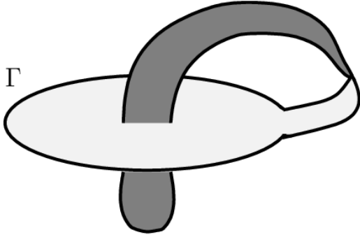
An area minimizing disk might have transverse self intersections.
