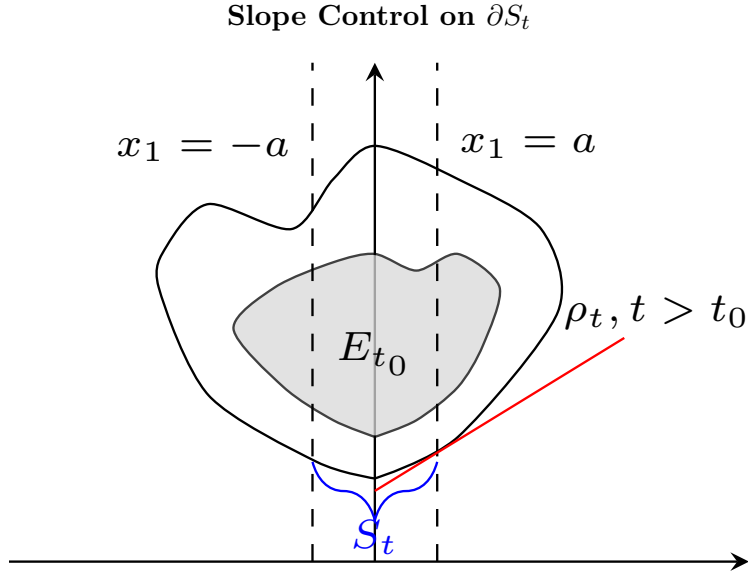
FIGURE 3.2. In order for \rho_t to properly enclose E_{t_0} for t > t_0 , the tangent line must have a uniformly small slope on \partial S_t .
