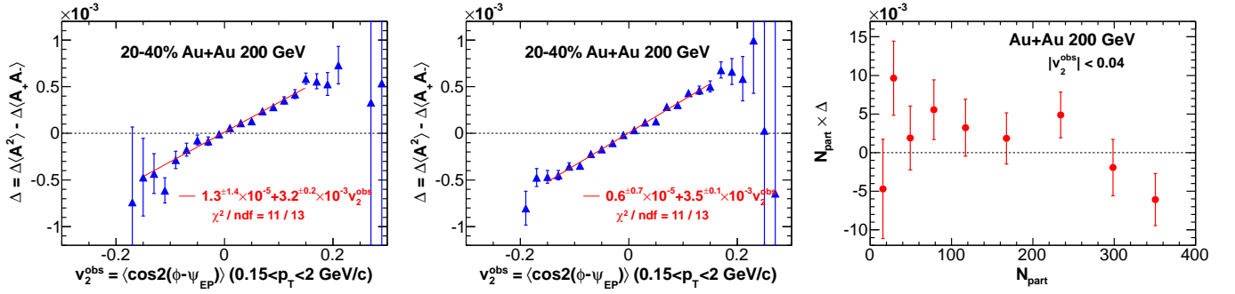
FIG. 13: (Color online) \Delta = \langle A^2 \rangle - \langle A_+ A_- \rangle as a function of v_2^{\text{obs}} , the event-by-event elliptical anisotropy of particle distributions relative to the second-harmonic event plane reconstructed from TPC tracks (left panel) and the first harmonic event plane reconstructed from the ZDC-SMD neutron signals (middle panel), in 20-40% central Au+Au collisions. Right panel: Average \Delta for events with |v_2^{\text{obs}}| < 0.04 relative to the TPC event plane as a function of centrality. The error bars are statistical only.
