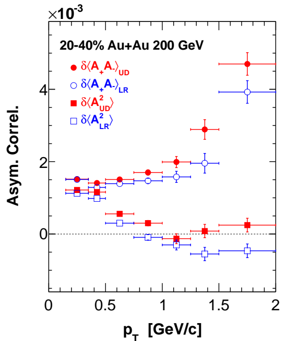
FIG. 5: (Color online) The p_T dependence of the charge asymmetry dynamical correlations, \delta\langle A^2 \rangle , and the positive and negative charge asymmetry correlations, \delta\langle A_+A_- \rangle . The data are from 20-40% central Au+Au collisions. The asymmetries are calculated between hemispheres separated by the event plane (UD) and between those separated by the plane perpendicular to the event plane (LR). The error bars are statistical only.
