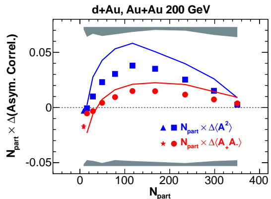
FIG. 4: (Color online) The correlation differences \Delta\langle A^2 \rangle = \delta\langle A_{\text{UD}}^2 \rangle - \delta\langle A_{\text{LR}}^2 \rangle and \Delta\langle A_+ A_- \rangle = \delta\langle A_+ A_- \rangle_{\text{UD}} - \delta\langle A_+ A_- \rangle_{\text{LR}} , scaled by the number of participants N_{\text{part}} , as a function of N_{\text{part}} . The error bars are statistical, and the systematic uncertainties are shown in the shaded bands (upper band for \Delta\langle A_+ A_- \rangle and lower band for \Delta\langle A^2 \rangle ). Also shown as the lines are the linear-extrapolated values of \Delta\langle A^2 \rangle and \Delta\langle A_+ A_- \rangle corresponding to a perfect event-plane resolution. The star and triangle depict the d+Au results.
