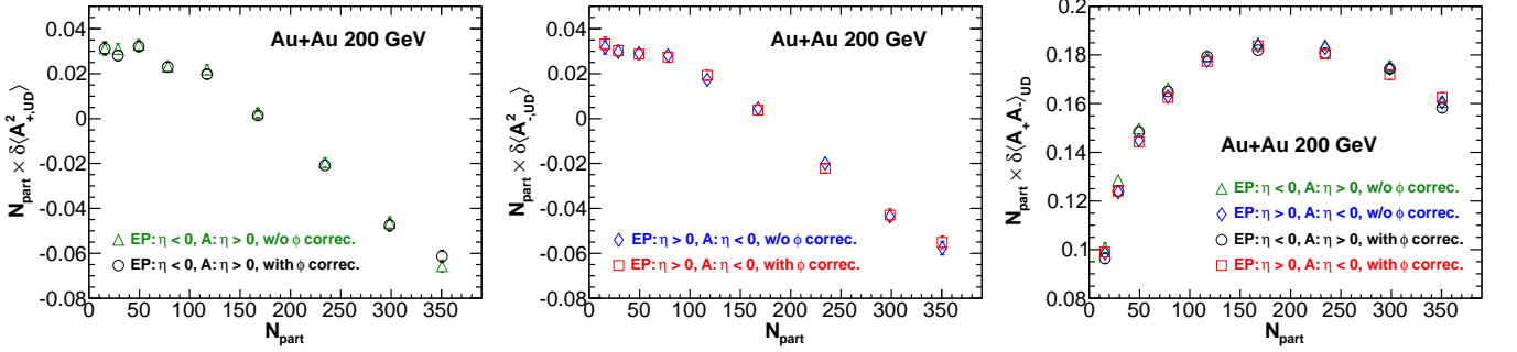
FIG. 21: (Color online) The statistical and detector effect subtracted asymmetry correlations, \delta \langle A_{+,LR}^2 \rangle (left panel), \delta \langle A_{-,LR}^2 \rangle (middle panel), and \delta \langle A_+ A_- \rangle_{LR} (right panel), multiplied by the number of participants N_{part} , before and after the corrections for the \phi -dependent acceptance \times efficiency. This figure corresponds to Fig. 18. The error bars are statistical only.
