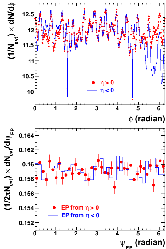
FIG. 16: (Color online) Upper panel: Positively charged particle multiplicity distributions versus the azimuthal angle, \phi , in 30-40% central Au+Au collisions. The data are shown separately for \eta > 0 and \eta < 0 . The magnetic polarities of the STAR magnet have been summed and the p_T is integrated over the range 0.15 < p_T < 2 GeV/c. The inverse of these distributions, properly normalized, were used to correct for the track efficiency versus \phi . Lower panel: Reconstructed event-plane azimuthal angle distributions in 30-40% central Au+Au collisions. Particles within 0.15 < p_T < 2 GeV/c from \eta < 0 and \eta > 0 were used separately to reconstruct the EP. The error bars are statistical only.
