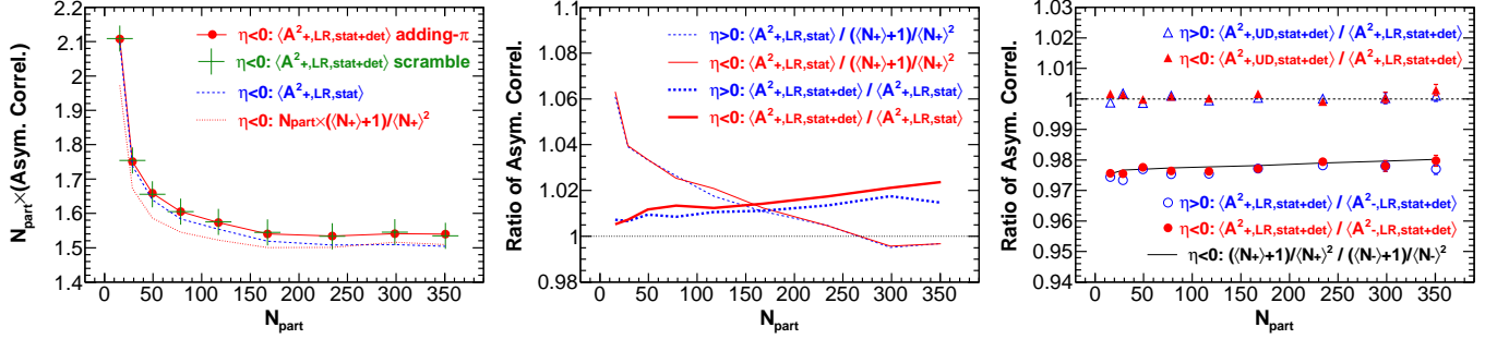
FIG. 19: (Color online) Left panel: Statistical fluctuation and detector effects in the charge asymmetry variance (multiplied by the number of participants N_{part} ) from the \eta < 0 region. The dotted curve shows the 1/N approximation using Eq. (B1), the dashed curve shows the statistical fluctuations \langle A_{+,LR,stat}^2 \rangle obtained by the “50-50” method (see the text). The solid curve connecting the solid points shows the net effect of the statistical fluctuations and detector non-uniformities, \langle A_{+,LR,stat+det}^2 \rangle , obtained by the adding- \pi method, and the crosses shows the same but obtained from the “scramble” method. See the text for details. Middle panel: The statistical fluctuation effects relative to the 1/N approximation (thin curves) and the effects due to the imperfect detector (thick curves). The dashed curves are for the region \eta > 0 and the solid curves are for \eta < 0 . Right panel: The ratios of the statistical fluctuation and detector effects \langle A_{+,LR,stat+det}^2 \rangle / \langle A_{+,LR,stat}^2 \rangle and \langle A_{+,UD,stat+det}^2 \rangle / \langle A_{+,LR,stat+det}^2 \rangle , separately for the \eta > 0 and \eta < 0 regions. The \phi -acceptance correction was applied for the results in this figure. The error bars are statistical only.
