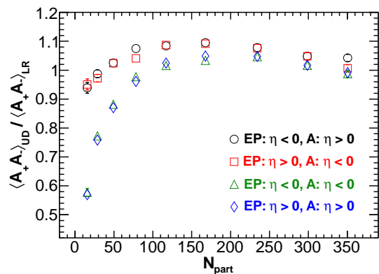
FIG. 17: (Color online) The relative charge asymmetry correlations, \langle A_+ A_- \rangle_{UD} / \langle A_+ A_- \rangle_{LR} , as a function of the number of participants, N_{part} , for four combinations of \eta ranges used for EP reconstruction and asymmetry calculation. The error bars are statistical only.
