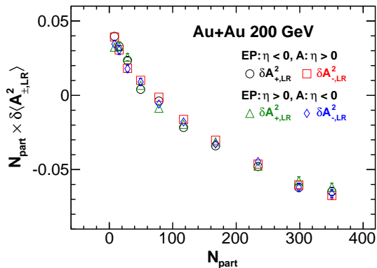
FIG. 22: (Color online) Dynamical charge asymmetry variance after removing the statistical and detector effects, \delta\langle A_{\pm,LR}^2 \rangle = \langle A_{\pm,LR}^2 \rangle - \langle A_{\pm,LR,stat+det}^2 \rangle , scaled by the number of participants N_{part} . The results are consistent between positive and negative \eta regions and between positive and negative charges. Error bars are statistical only.
