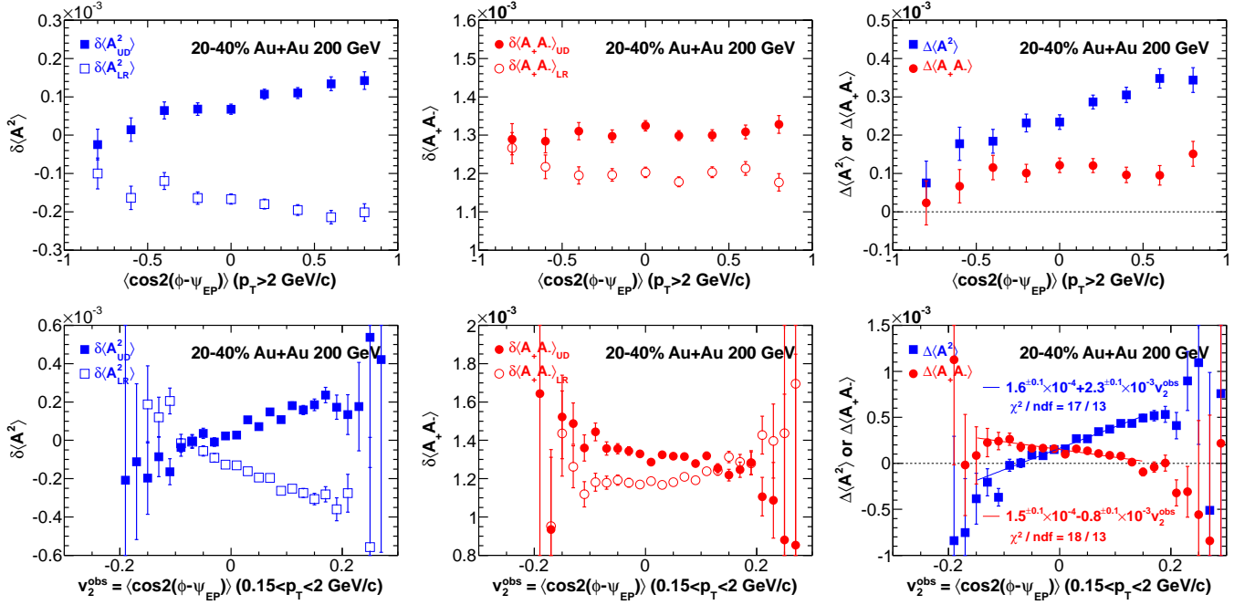
FIG. 7: (Color online) The charge asymmetry correlations \delta\langle A^2 \rangle (left panels) and \delta\langle A_+ A_- \rangle (center panels), and correlation differences \Delta\langle A^2 \rangle = \delta\langle A_{UD}^2 \rangle - \delta\langle A_{LR}^2 \rangle and \Delta\langle A_+ A_- \rangle = \delta\langle A_+ A_- \rangle_{UD} - \delta\langle A_+ A_- \rangle_{LR} (right panels), as a function of the azimuthal ellipticity of high- p_T ( p_T > 2 GeV/c) particles (upper panels) and low- p_T ( p_T < 2 GeV/c) particles (lower panels). Data are from 20-40% Au+Au collisions. The particle p_T range of 0.15 < p_T < 2 GeV/c is used for both EP construction and asymmetry calculation. Error bars are statistical.
