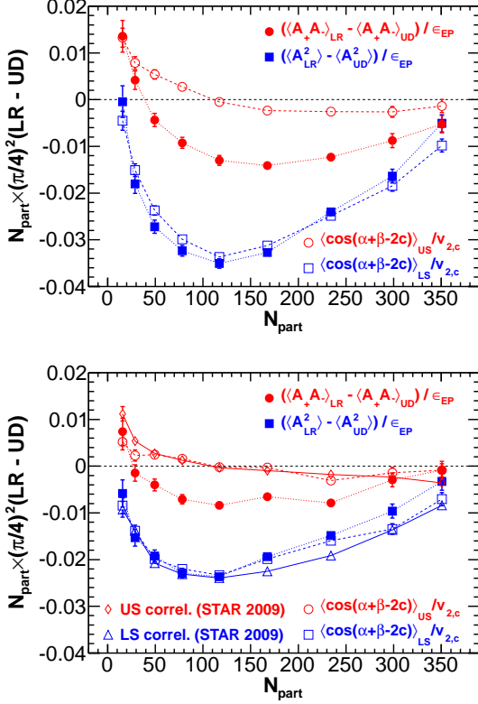
FIG. 15: (Color online) The correlation differences, \langle A_{LR}^2 \rangle - \langle A_{UD}^2 \rangle and \langle A_+A_- \rangle_{LR} - \langle A_+A_- \rangle_{UD} , scaled by the number of participants (\pi/4)^2 N_{\text{part}} . Also shown are \langle \cos(\phi_\alpha + \phi_\beta - 2\phi_c) \rangle / v_{2,c} \approx \langle \cos(\phi_\alpha + \phi_\beta - 2\psi_{RP}) \rangle of same- and opposite-sign particle pairs ( \alpha and \beta ) calculated from particles used for the charge asymmetry correlations with particle c from those used for EP construction. The upper panel shows the default results where particles are divided according to \eta ; the lower panel shows results with particles divided randomly into two halves and compared to published correlators (STAR 2009 [14, 15]). The error bars are statistical only.
