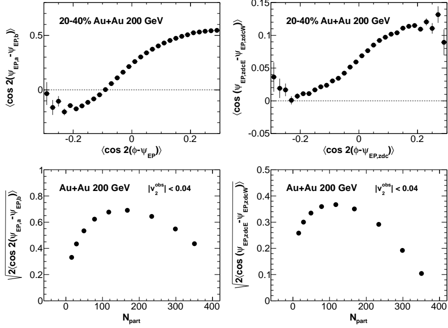
FIG. 25: The TPC second-harmonic (upper left) and ZDC-SMD first harmonic (upper right) event-plane resolution as a function of v_2^{\text{obs}} in 20-40% central Au+Au collisions. The TPC second-harmonic (lower left) and ZDC-SMD first harmonic (lower right) event-plane resolution for events with |v_2^{\text{obs}}| < 0.04 as a function of centrality. The error bars are statistical only.
