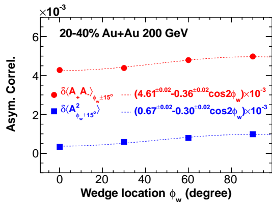
FIG. 9: (Color online) Charge multiplicity asymmetry correlations as a function of the wedge location, \phi_w , in 20-40% central Au+Au collisions. The wedge size is 30^\circ . The curves are the characteristic \cos(2\phi_w) to guide the eye. The error bars are statistical only.
