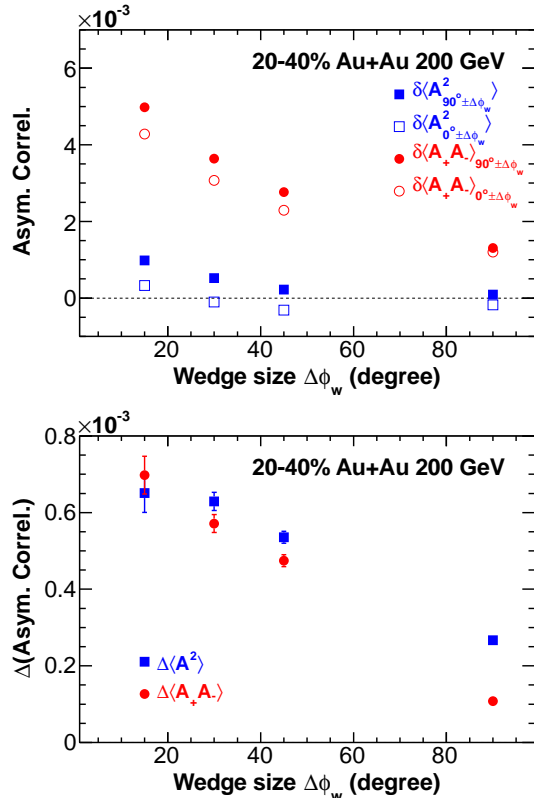
FIG. 8: (Color online) The wedge size dependences of charge multiplicity asymmetry correlations (upper panel), and their differences between out-of-plane and in-plane, \Delta\langle A_{\Delta\phi_w}^2 \rangle and \Delta\langle A_+ A_- \rangle_{\Delta\phi_w} (lower panel) for 20-40% central Au+Au collisions. The error bars are statistical only.
