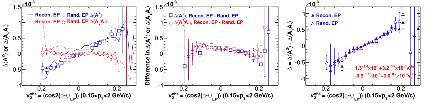
FIG. 14: (Color online) Left panel: \Delta\langle A^2 \rangle and \Delta\langle A_+A_- \rangle as a function of v_2^{\text{obs}} with a random EP in 20-40% Au+Au collisions. The lines depict the results with reconstructed EP from Fig. 7 lower right panel for comparison. Middle panel: The differences in \Delta\langle A^2 \rangle and \Delta\langle A_+A_- \rangle between the reconstructed EP and random EP results, respectively. Right panel: \Delta = \Delta\langle A^2 \rangle - \Delta\langle A_+A_- \rangle as a function of v_2^{\text{obs}} with a random EP (open triangles). The solid triangles are results with reconstructed EP from Fig. 13 left panel for comparison. Error bars are statistical.
