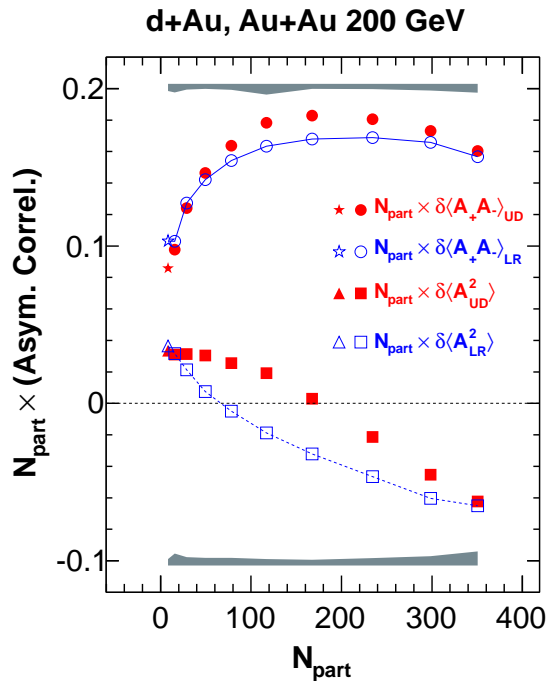
FIG. 3: (Color online) Centrality dependences of the charge asymmetry dynamical correlations, \delta\langle A^2 \rangle , and the positive and negative charge asymmetry correlations, \delta\langle A_+ A_- \rangle . The asymmetries are calculated between hemispheres separated by the event plane (UD) and between those separated by the plane perpendicular to the event plane (LR). The asymmetry correlations are multiplied by the number of participants N_{\text{part}} . The error bars are statistical only. The upper (lower) shaded band shows half of the systematic uncertainty in the \delta\langle A_+ A_- \rangle ( \delta\langle A^2 \rangle ); the larger of the UD and LR systematic uncertainties is drawn. The stars and triangles depict the d+Au results.
