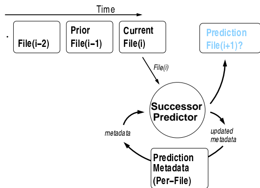
Figure 1. On-line successor prediction.
