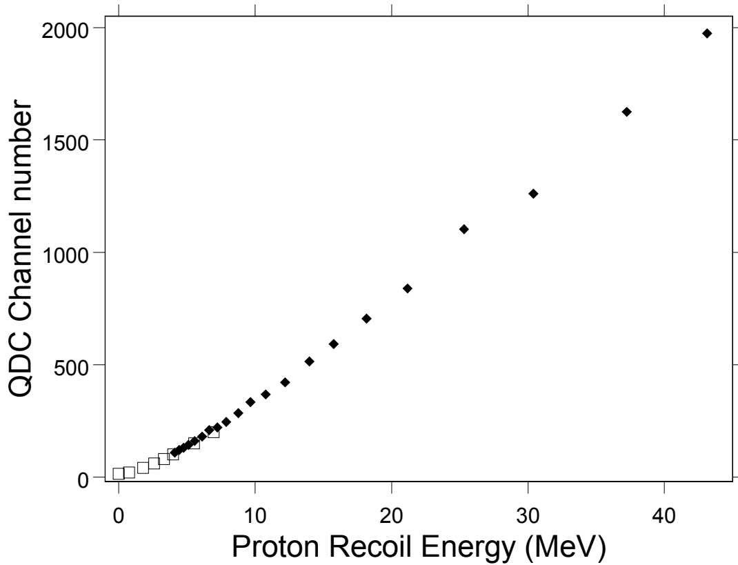
FIG. 2. Pulse-height-to-energy calibration of the charge-integrating analog-to-digital converter. The open, square symbols show the fit to the Compton-edge data, and the closed, diamond-shaped symbols show the data from the maximum-recoil method.
