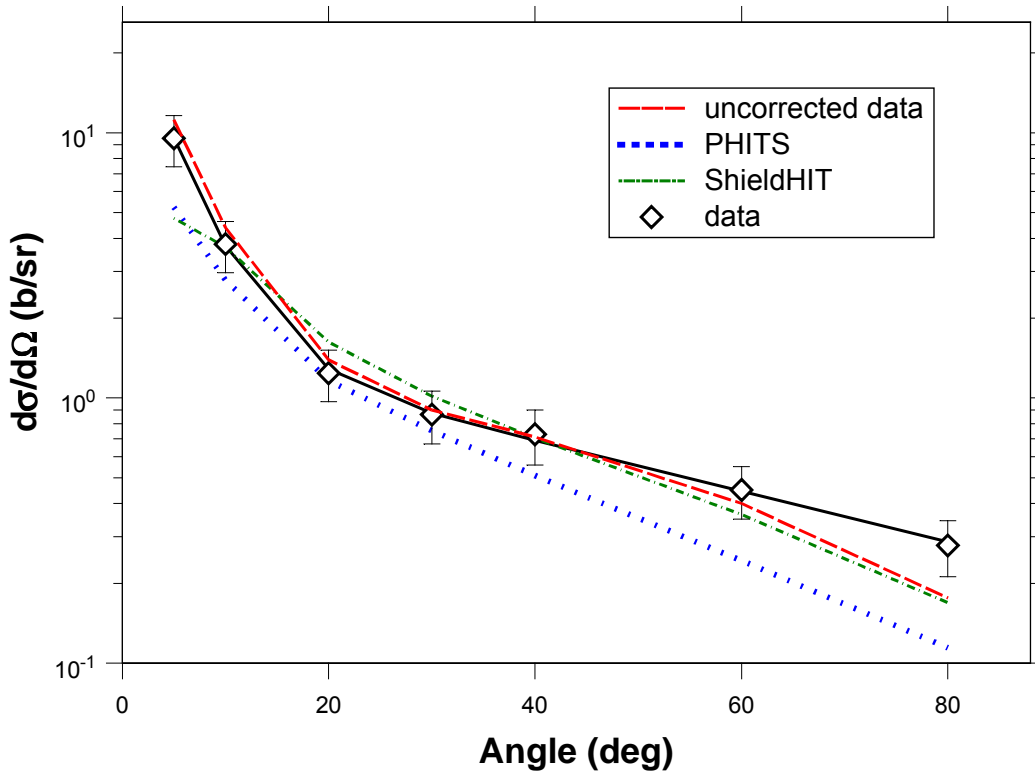
FIG. 8. (Color online) Angular distribution for the 290 MeV/nucleon C + marsbar system. The data are shown with the symbols. The error bars include both systematical and statistical uncertainties. The dashed (red) line shows the data without corrections for attenuation and for production from non-target materials. Results from PHITS and SHIELD-HIT calculations are shown with the dotted (blue) and dot-dashed (green) lines, respectively. The solid line comes from a fit explained in the text.
