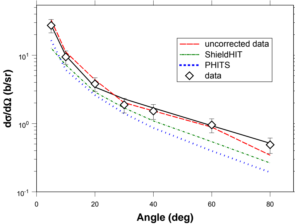
FIG. 10. (Color online) Angular distribution for the 600 MeV/nucleon Ne + marsbar system. The data are shown with the symbols. The error bars include both systematical and statistical uncertainties. The dashed (red) line shows the data without corrections for attenuation and for production from non-target materials. Results from PHITS and SHIELD-HIT calculations are shown with the dotted (blue) and dot-dashed (green) lines, respectively. The solid line comes from a fit explained in the text.
