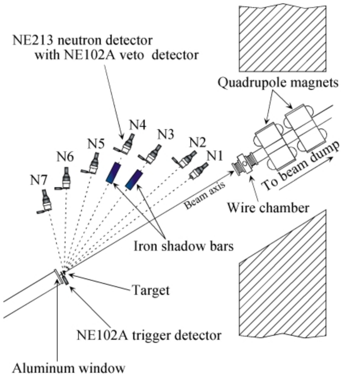
FIG. 1. A schematic diagram of the experimental setup on the SB3 beam course at HIMAC. The quadrupole magnets are positioned at a concrete shielding wall separating the target hall from the shield room where the beam dump was located.
