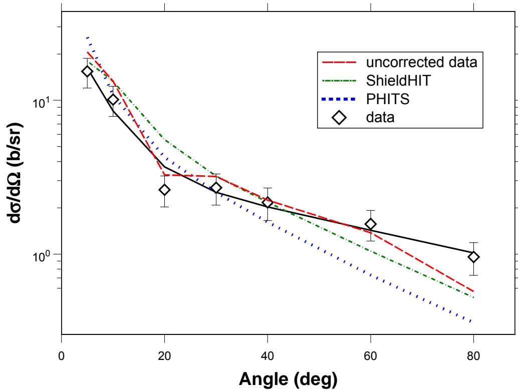
FIG. 9. (Color online) Angular distribution for the 400 MeV/nucleon Ne + ISS wall system. The data are shown with the symbols. The error bars include both systematical and statistical uncertainties. The dashed (red) line shows the data without corrections for attenuation and for production from non-target materials. Results from PHITS and SHIELD-HIT calculations are shown with the dotted (blue) and dot-dashed (green) lines, respectively. The solid line comes from a fit explained in the text.
