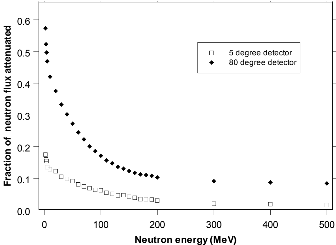
FIG. 4. An estimation of the fraction of neutron flux that does not make it to the neutron detector due to absorption and out-scattering in the marsbar target and other intervening materials between the target and detector. The open, square symbols show the fraction lost from the detector at 5°, and the closed, diamond-shaped symbols show the fraction lost from the detector at 80°.
