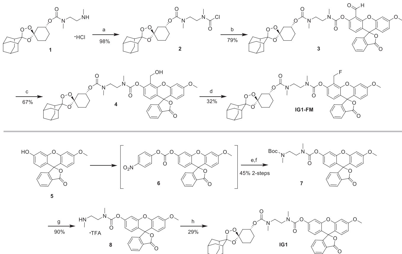
Scheme 2. Synthesis of IG1-FM and control probe IG1. Reagents and conditions: (a) \text{COCl}_2 (15 wt.% in toluene), \text{NEt}_3 , \text{CH}_2\text{Cl}_2 , 0^\circ\text{C} to rt, 1.5 h; (b) Compound S1, DMAP, \text{Et}_3\text{N} , \text{CH}_2\text{Cl}_2 , rt, 4.5 h; (c) \text{NaBH}_4 , \text{THF}/\text{EtOH} (1:1), -78^\circ\text{C} to 0^\circ\text{C} , 3.5 h; (d) Deoxo-Fluor, 0^\circ\text{C} to rt, 17 h. (e) 4- \text{NO}_2\text{PhOC(O)Cl} , \text{Et}_3\text{N} , \text{THF} , 0^\circ\text{C} to rt, 1 h; (f) tert-butyl methyl[2-(methylamino)ethyl]carbamate, 0^\circ\text{C} , 15 min; (g) \text{TFA}/\text{CH}_2\text{Cl}_2 (1:1), 0^\circ\text{C} , 40 min; (h) Compound S2 \text{Et}_3\text{N} , \text{DMF} , 0^\circ\text{C} , 2 h 40 min.
