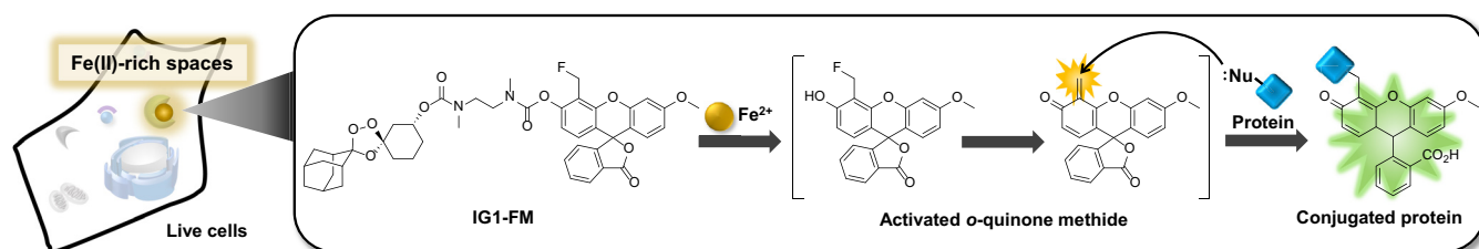
Scheme 1. Design and chemical structure of IG1-FM, a dual tandem ABS and labeling probe for fluorescence detection of labile Fe(II).
