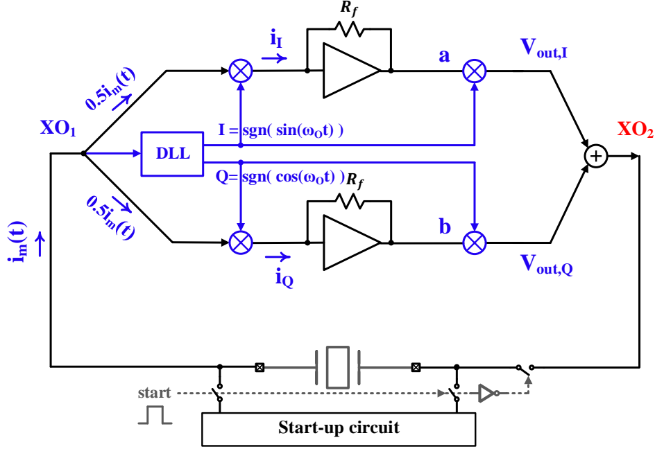
Figure 4.11: Principle of operation of the ULP XO with I/Q frequency conversion.
