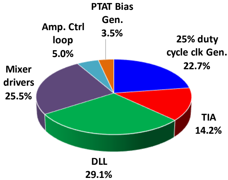
Figure 4.31: Power contribution of main blocks of the ULP 32kHz XO.
