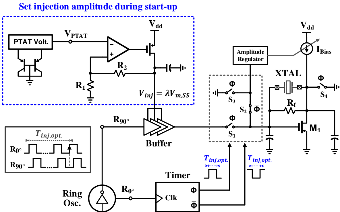
Figure 3.12: Block diagram of the proposed fast start-up crystal oscillator.
