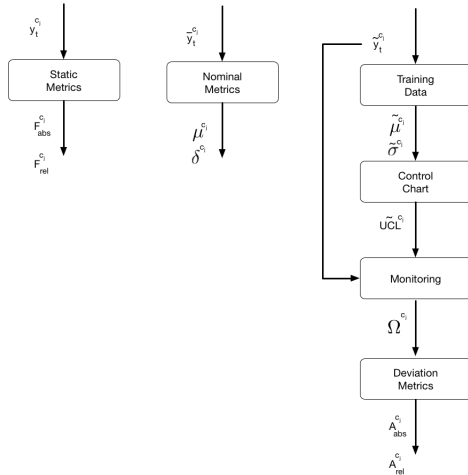
Figure 4.9: Inside-Out layer: computation of the quality metrics
